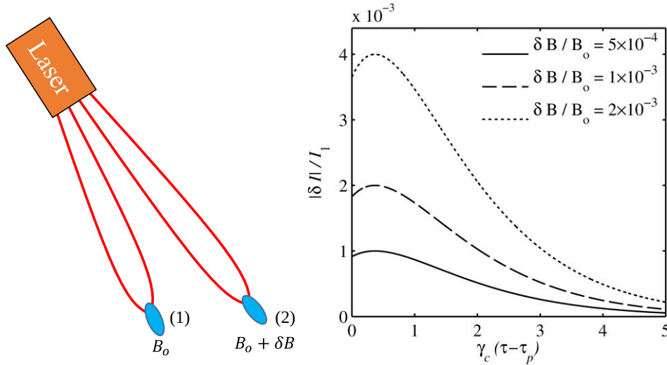
Figure 7: Fractional difference in the wakefield intensity for various fractional differences in the magnetic field \delta B/B_o . The pump pulse has duration \tau_p = 500 psec, spot size 1 mm, and energy 100 mJ. The differences in magnetic field and corresponding intensities are from two nearby locations.
