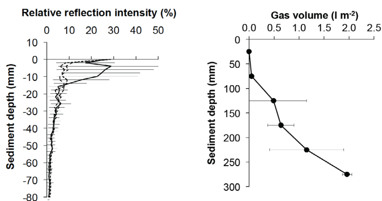
Fig. 1. Left: Distribution of oxygen bubbles in St. Joseph Bay sediment, Florida. Dotted lines present distribution under dark conditions. Right: Methane profiles in sediment affected by groundwater seepage. Free methane gas builds up below 10 cm depth.
