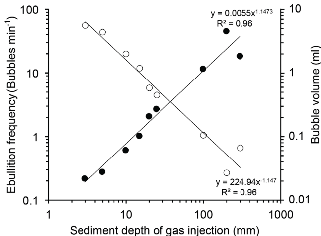
Fig. 2. The frequency (open circles) and volume (solid circles) of bubbles released after injection of gas at 1.24 ml min -1 at different sediment of nearshore marine sand.
