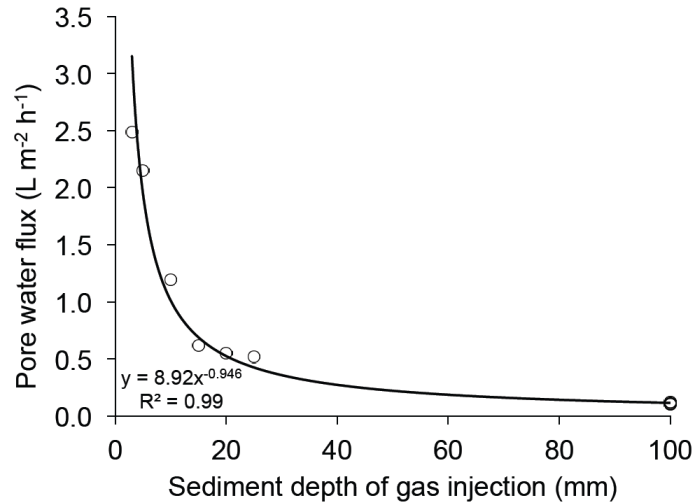
Fig. 4. Pore water flux resulting from gas injection at different sediment depth at a constant rate of 1.2 \text{ ml min}^{-1} . At shallow injection depth, the ebullition was more effective for increasing interfacial solute flux compared to the deeper injection.
