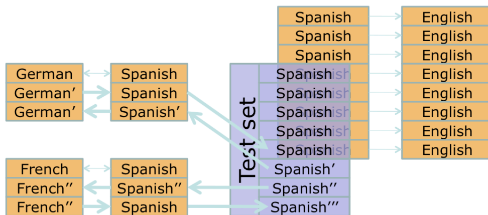
Figure 4.1: Pivoting technique for paraphrase generation. For a Spanish-to-English translation model, which encounters unknown source language (Spanish) phrases, augment the model by pivoting through other languages such as French or German. This requires translation models to and from these pivot languages, which are typically generated from sentence-aligned parallel texts. However, parallel texts are a limited resource.
