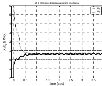
Left and Right vortex breakdown time history
