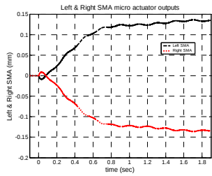
Left and Right SMA control loop output time history
