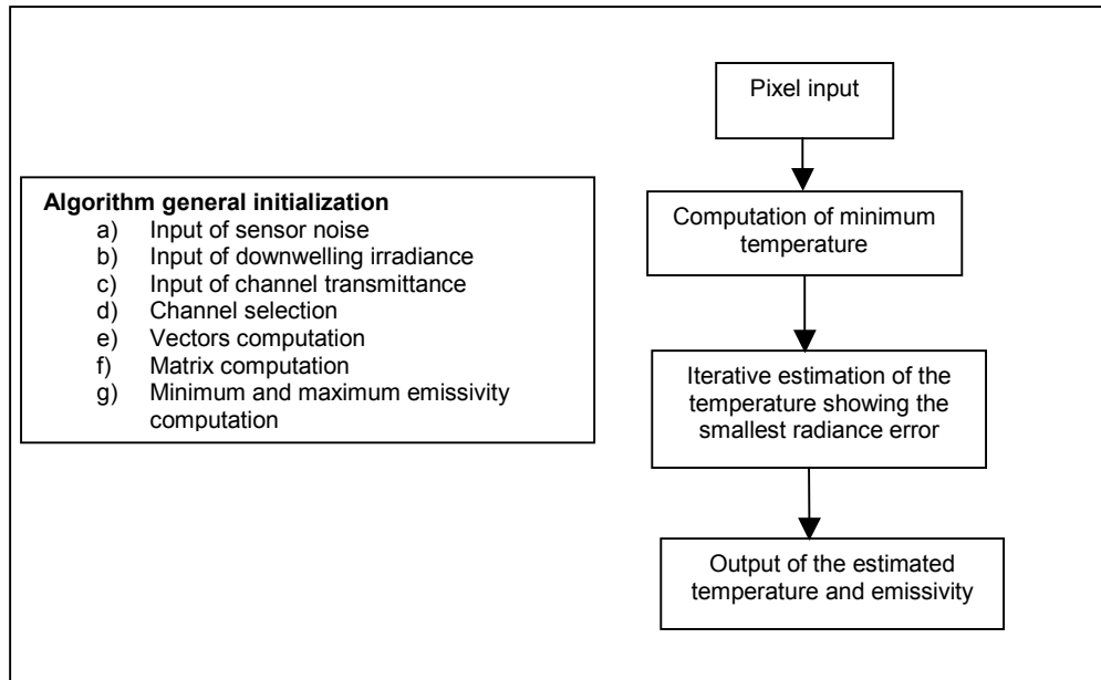
Figure 3: Program flow for the proposed algorithm
