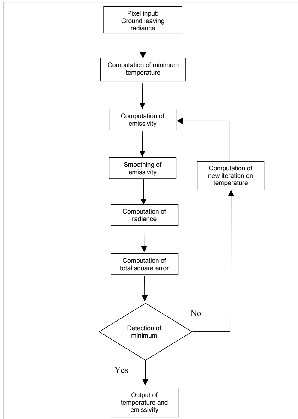
Figure 4: Detailed algorithm of the pixel processing
