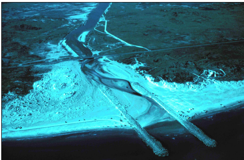
Figure 13. Aerial photo of the Fish Pass, Mustang Island, TX (1983) showing its configuration and the sediment accumulation in the channel
