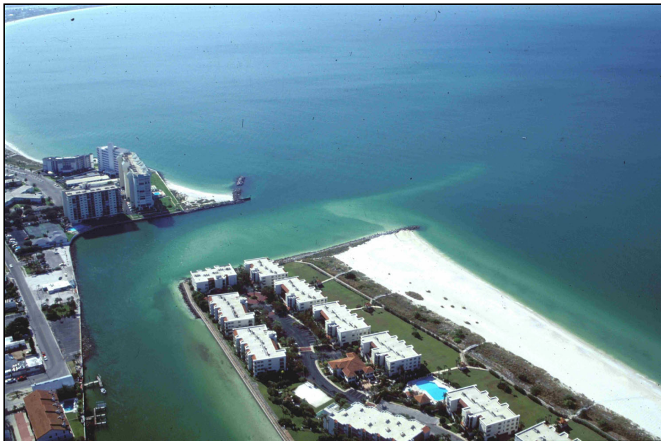
Figure 2. Blind Pass, 1999, an example of an unstable wave-dominated inlet
