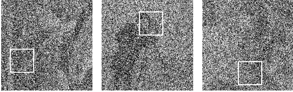
Fig. 5. The images of “Lena”, “Cameraman”, and “Barbara” (from left to right) corrupted by impulsive noise with noise level of 70%.
