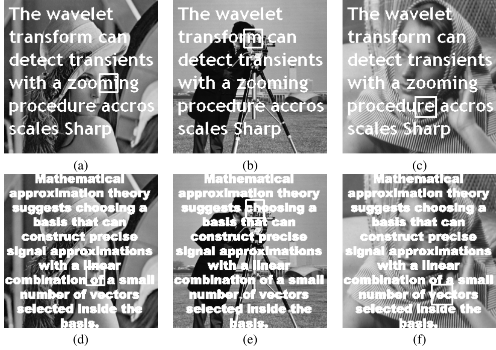
Fig. 2. The test images superposed by “Text 1” (the first row) and the “Text 2” (the second row). The square region in each image is the part of the corresponding image zoomed in.
