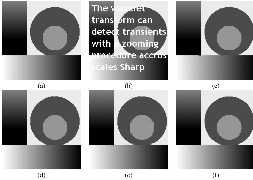
Fig. 1. Performance of various inpainting algorithms for a cartoon image with text. (a) the original test image; (b) the test image with text; inpainted images by (c) SF (PSNR=37.38 dB); (d) SF-LDCT (PSNR=37.37 dB); (e) MCA (PSNR=37.04 dB); and (f) the proposed algorithm (PSNR=39.96 dB), respectively.
