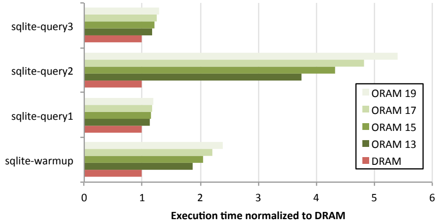
Figure 7.6: Simulated SQLite Performance. We simulated the performance of SQLite running on a timing model of PHANTOM with and without ORAM. We assume a 1MB L2 cache, 16KB icache, 32KB dcache and an extra buffer for 8 ORAM blocks (32KB).
