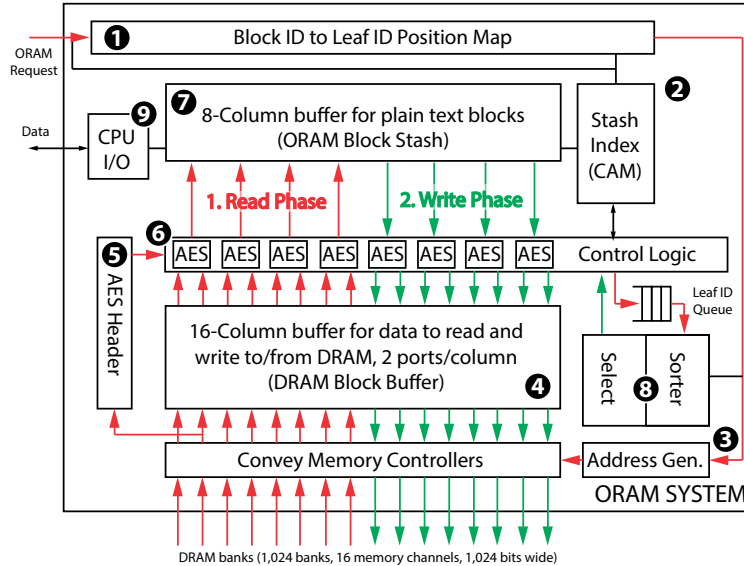
Figure 5.1: Overview of the ORAM controller. The arrows represent the data flow during the two phases of the Path ORAM algorithm.
