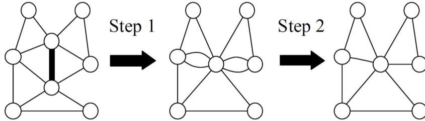
Figure 2.1: Face clustering [18]
