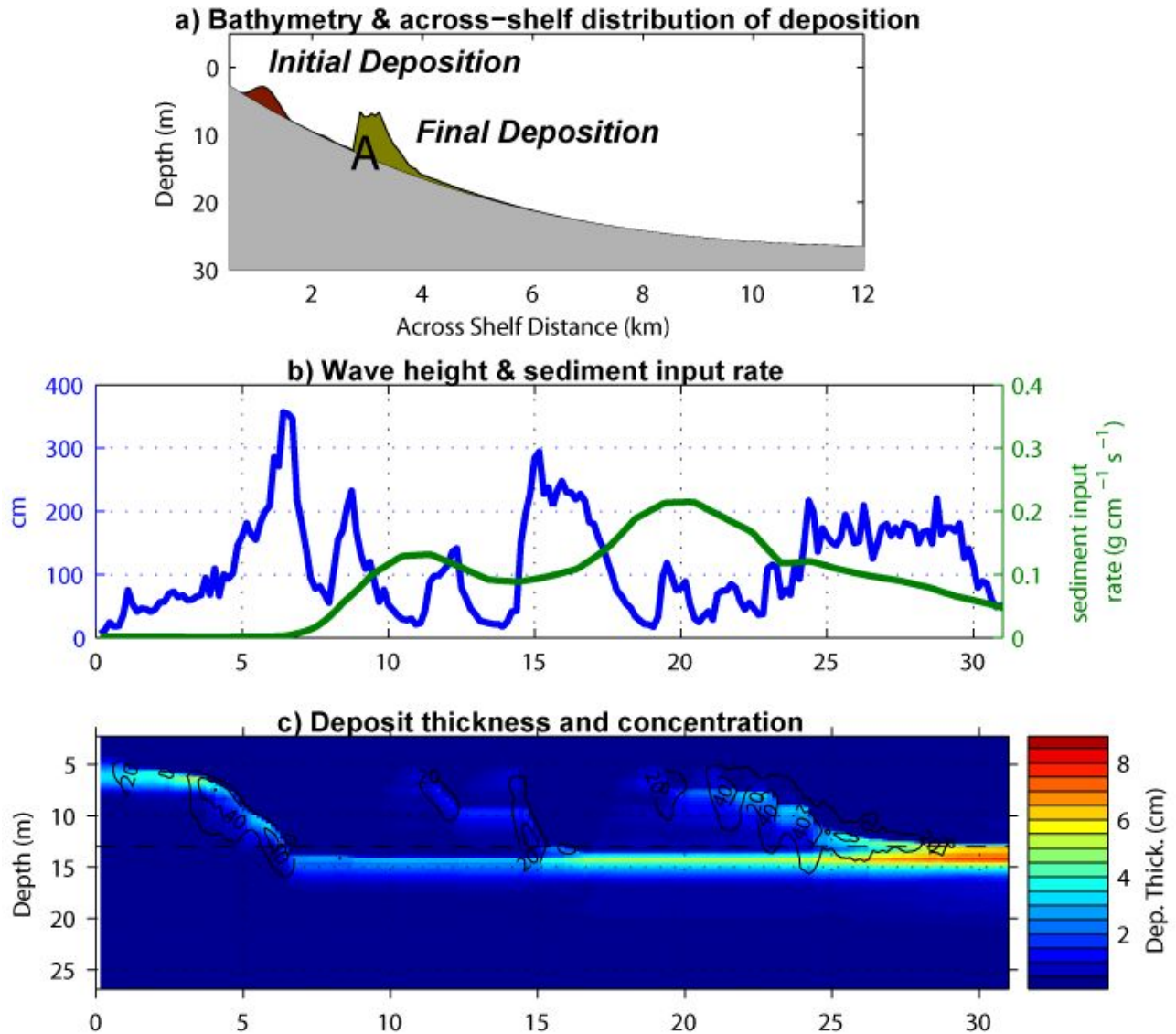
Figure 2. Model Runs for the Po prodelta. a) Bathymetry, initial and final distribution of sediment deposition thickness. The vertical scale for the sediment deposition has been exaggerated by a factor of 100. The location of the tripod is indicated by A. b) Wave height (left y-axis) and sediment input rate (right y-axis, proportional to river discharge). c) Temporal and depth dependence of deposition (color scale) and suspended sediment concentration within the wave boundary layer (contours with units of g/l). A dashed line at 13 m depth depicts the tripod location. Due to the slightly smaller waves compared to the Eel and significantly shorter wave period at the Po site wave-supported turbidity currents were able to transport sediment to the 13 to 15 m isobath where it was deposited
