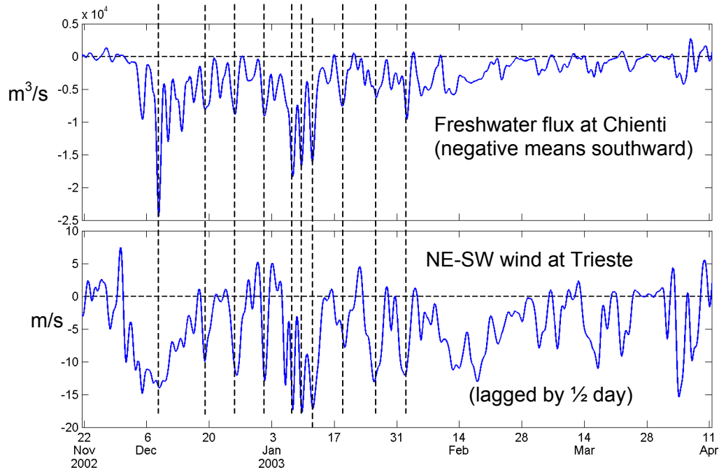
Figure 3. Freshwater flux at Chienti (top panel) and NE-SW winds at Trieste (lower panel). The freshwater flux matches the seasonally averaged freshwater inputs into the northern Adriatic, although there are major spikes in the freshwater flux that are due to the winds rather than freshwater flow events (examples indicated by vertical dashed lines). The strong Bora events (downward spikes in wind velocity) are critical agents for along-coast sediment transport.
