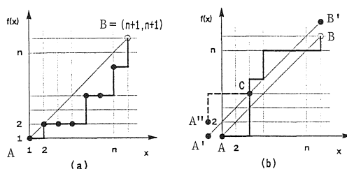
FIGURE 2. Monotonic mapping equivalence to the path problem
