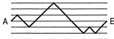
FIGURE 1. The path problem
