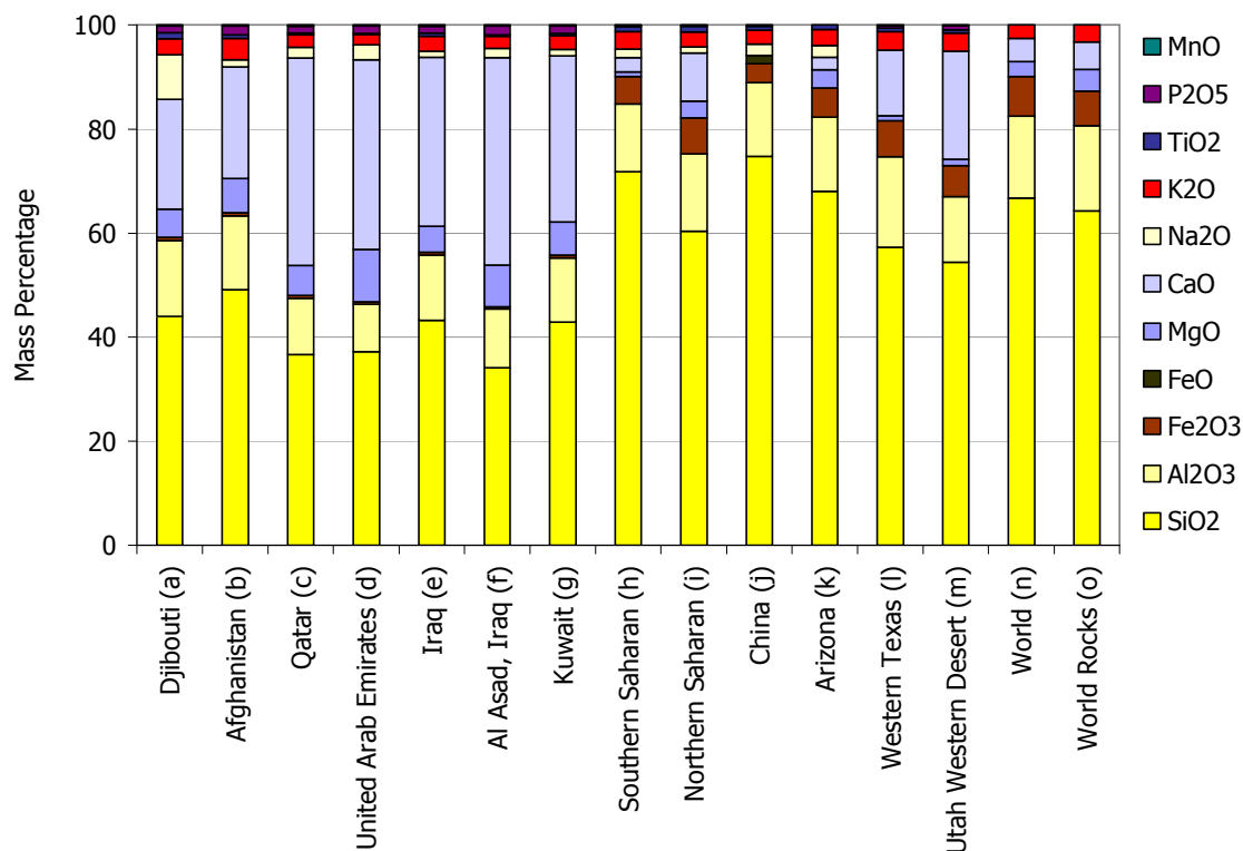
Figure 4-8. Comparison of dust samples from the Middle East, Sahara, China, U.S., world average dust, and world rocks. In the case of the EPMSP samples, mean TSP results are shown, from (a) Djibouti; (b) Bagram and Khowst in Afghanistan; (c) Qatar; (d) UAE; (e) Balad, Baghdad, Tallil, Tikrit, and Taji in Iraq; (f) Al Asad in Iraq; (g) Northern, Central, Coastal, and Southern Kuwait; (h) average Southern Sahara [Goudie, 2006]; (i) average Northern Sahara [Goudie, 2006]; (j) average China [Goudie, 2006]; (k) Arizona [Goudie, 2006]; (l) Western Texas [Labban, 2004]; (m) Utah Western Desert [Labban, 2004]; (n) average world dust [Goudie, 2006]; and average world crustal rocks [Clarke, 1916].
