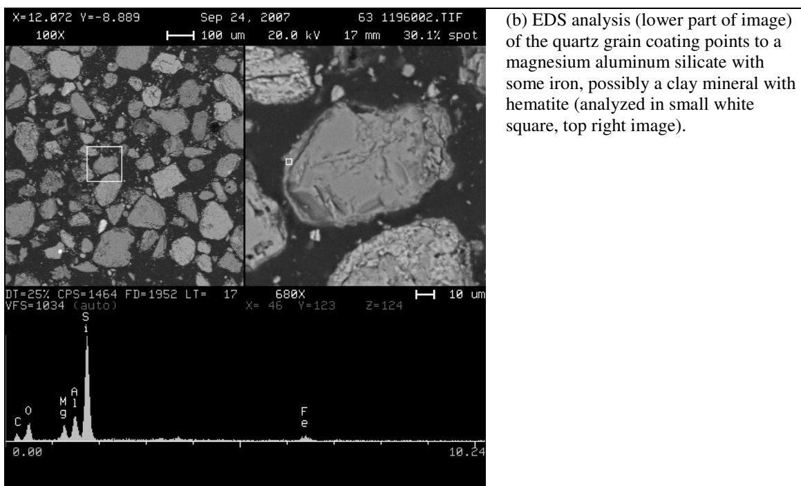
Figure 4-16. A polished section of sieved bulk dust sample from Coastal Kuwait showing compositional details of (a) a quartz grain and (b) its coating, consisting of a magnesium aluminum silicate clay, possibly montmorillonite and/or palygorskite.
