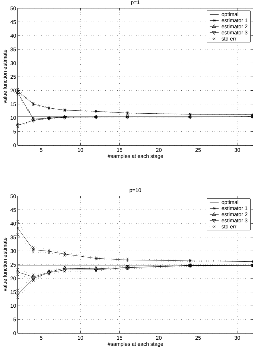
Figure 3.5: Convergence of value function estimate for the inventory control example case
