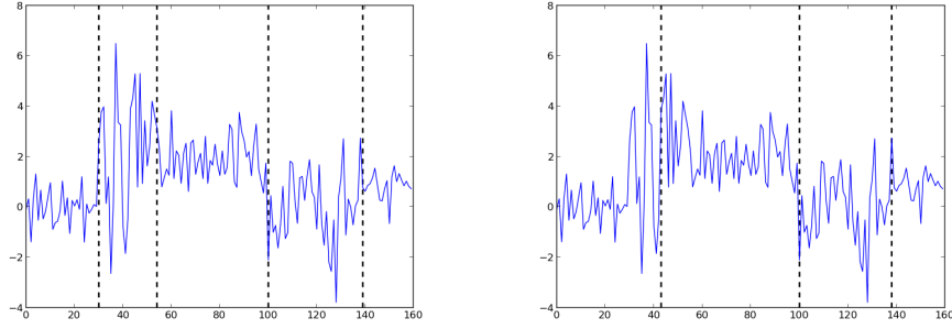
Figure 4: Five segments of discrete-mean Gaussian data with changing variance: an accurate segmentation by CHAMP (left) and an inaccurate segmentation using Fearnhead and Liu’s original algorithm (right) that misses a change in variance without a change in mean.
