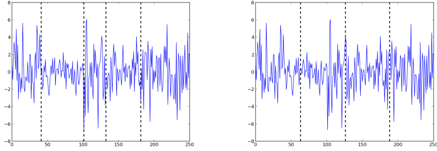
Figure 2: Five segments of mean-zero Gaussian data with changing variance: an accurate segmentation by CHAMP (left) and an inaccurate segmentation using Fearnhead and Liu’s original algorithm (right).
