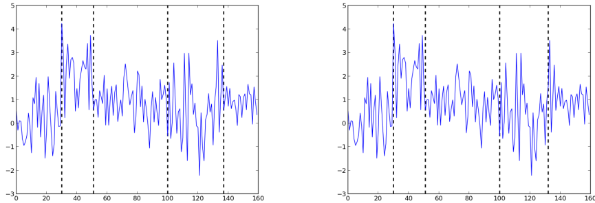
Figure 3: Five segments of discrete-mean Gaussian data with changing variance: an accurate segmentation by both CHAMP (left) and Fearnhead and Liu’s original algorithm (right). Note that the mean changes with every segment.
