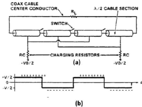
Figure 1. Two cycle frozen wave generator illustration. (a) Physical layout showing coaxial elements. (b) Static potential distribution showing polarity of each element in (a). (Reproduced from Forcier, et al., [5])
