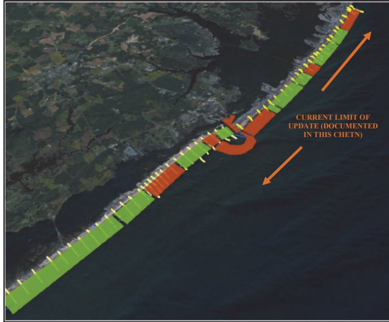
Figure 1. Extent of past sediment budgets (red = net loss; green = net gain).
