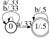
Figure 1: An unambiguous weighted finite automaton that cannot be determinized. 0 is the initial state and 1 the final state. The automaton accepts the set of strings (a^*b^*)^*ab^* .
