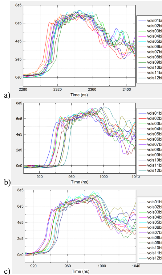
Figure 3. PFL output waveforms (vols) for representative shots in a) negative polarity (shot 0730), b) positive polarity with electrode spacers (shot 1086) and c) positive polarity with new electrode hardware (shot 1117).
