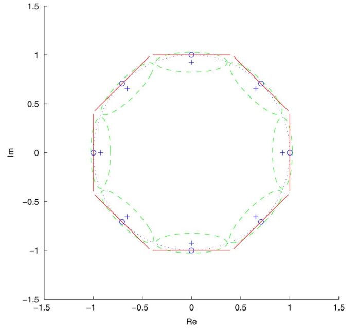
Fig. 6. Unconstrained and constrained estimates using the linearized projection algorithm. The unconstrained estimates are the set of dashed ellipses with means at + . The constrained estimates are shown as solid ellipses with means at o . The unit circle is drawn as the dotted line.
