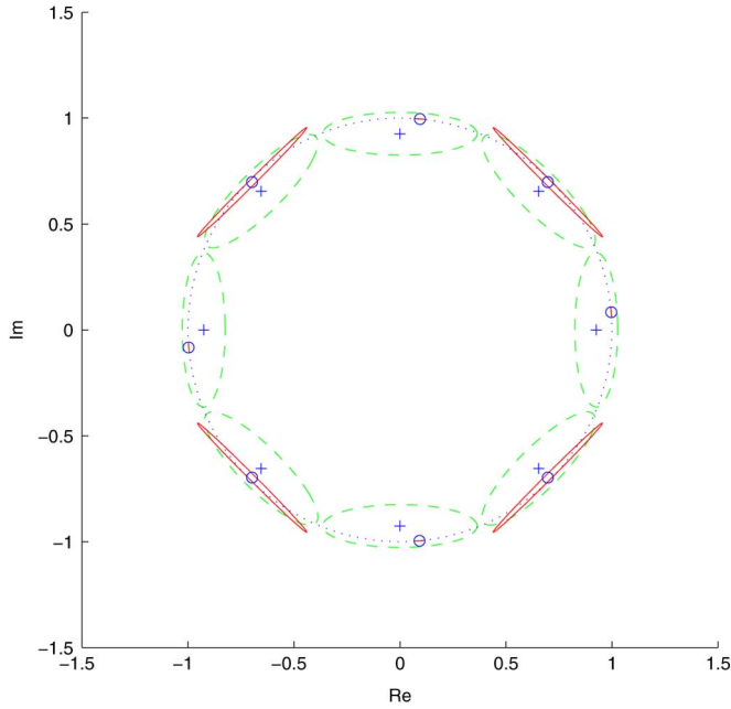
Fig. 5. Unconstrained and constrained estimates using the SCKF algorithm. The unconstrained estimates are the set of dashed ellipses with means at + . The constrained estimates are shown as solid ellipses (collapsed to short solid lines in some cases) with means at o . The unit circle is drawn with a dotted line.
