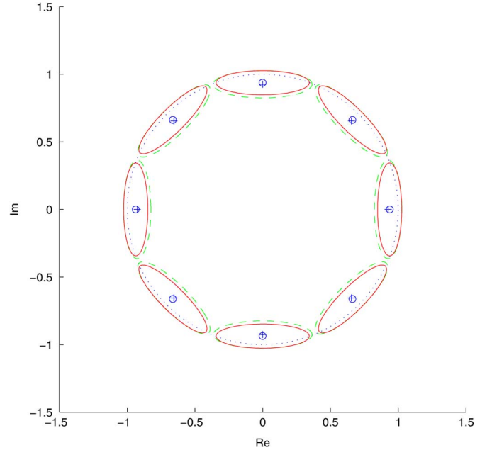
Fig. 7. Unconstrained and constrained estimates using the UT projection algorithm. The unconstrained estimates are the set of dashed ellipses with means at + . The constrained estimates are shown as solid ellipses with means at o . The unit circle is drawn with the dotted line.
