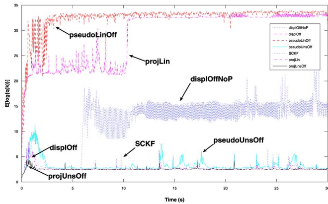
Fig. 11. Natural logarithm of the normalized state error for the different filters. pseudoLinOff and projLin have the largest means, with values about 30. displOffNoP lies in the middle with a mean of about 15. displOff , pseudoUnsOff , SCKF , and projUnsOff all have means of around 2.5.
