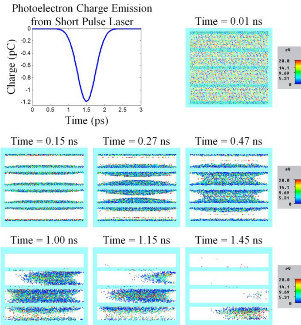
Figure 5. Photoelectrons created by short pulse laser type pulse shown at plane on top of microstrips. They originally travel upwards, as shown for 0.01 ns, then return to the top of the microstrips, create secondaries, and interact with the gate pulses (pores not modeled).
