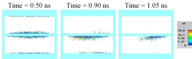
Figure 19. Evolution of electrons on top of microstrips for two strip with 8 kV phosphor and 150 V reverse bias.
