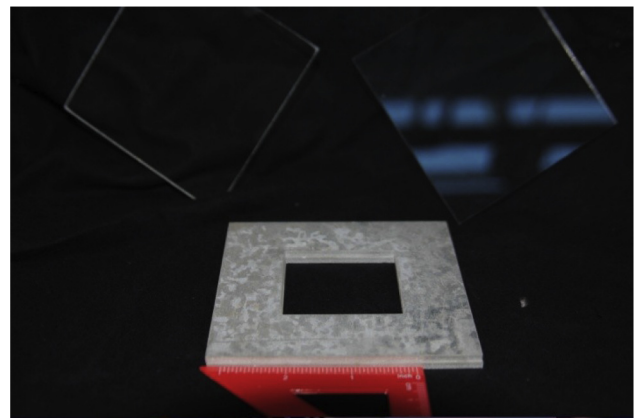
Fig. 1. Experimental setup. The glass and polycarbonate plates are sandwiched between two metal frames and clamped together at the outer edge.
