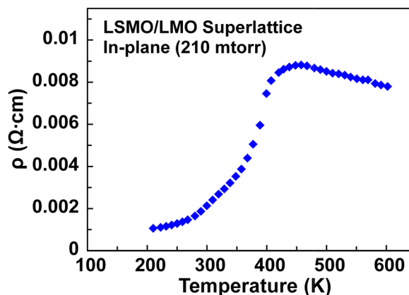
FIG. 10. Temperature-dependent in-plane resistivity of p-type LSMO/LMO superlattice.
