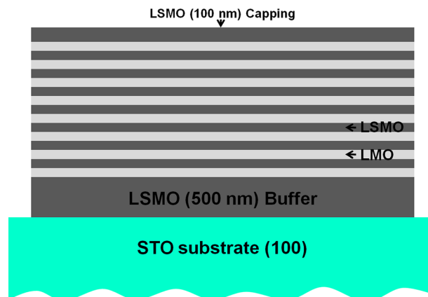
FIG. 4. Schematic of metallic LSMO (8 nm)/semiconducting LMO (8 nm) superlattice (\text{LSMO/LMO})_{51} structure grown by PLD.
