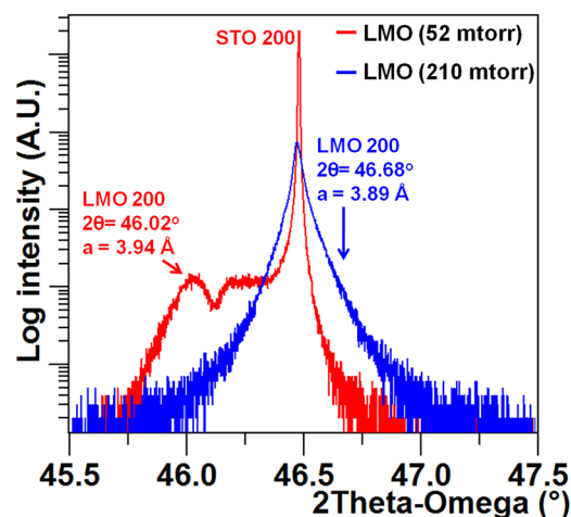
FIG. 3. XRD 2-theta-omega scan of an LMO on a STO (100) substrate confirming c-axis epitaxial behavior. The LMO grown at 52 mTorr partial oxygen pressure shows a distinguishing peak with a = 3.94 \text{ \AA} whereas the LMO grown at 210 mTorr peak overlaps with the STO peak.
