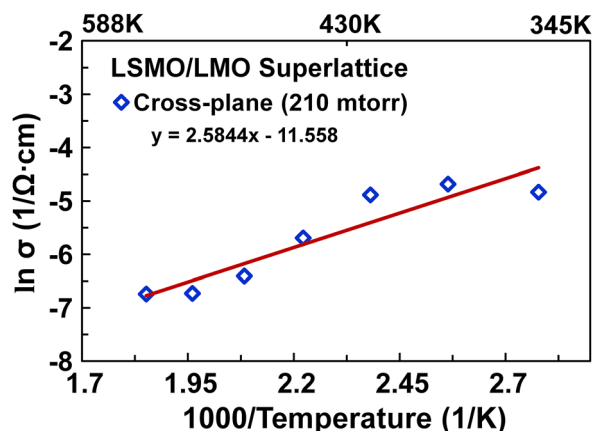
FIG. 13. Arrhenius plot of cross-plane LSMO/LMO superlattice electrical conductivity. The fitting extracted an effective barrier height of 223 \pm 11 meV.
