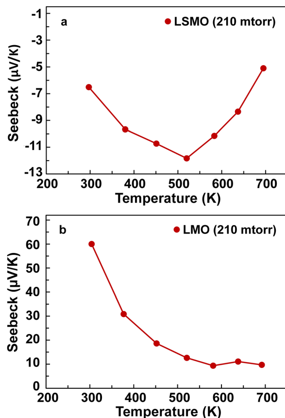
FIG. 7. (a) In-plane Seebeck measurement of LSMO showing that the Seebeck coefficient is consistent with metallic behavior with a magnitude of less than 15 \mu\text{V/K} and (b) in-plane Seebeck measurement of LMO validating p-type behavior with a room temperature Seebeck coefficient of 60 \pm 3 \mu\text{V/K} .
