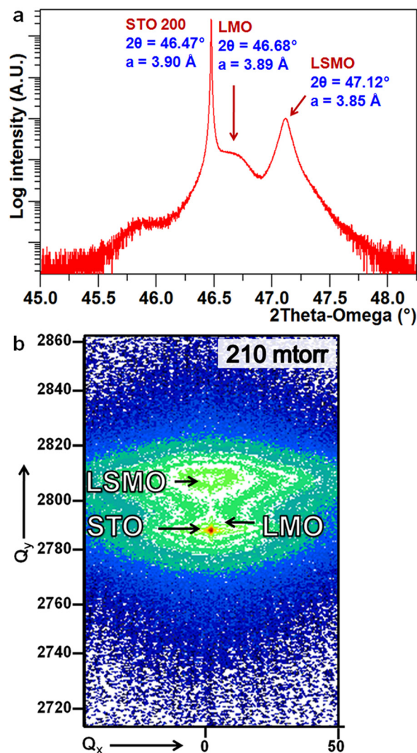
FIG. 5. (a) XRD 2-theta-omega scan of an LSMO/LMO superlattice on a STO (100) substrate confirming c-axis epitaxial behavior with LSMO FWHM ( 0.187^\circ ) and (b) 110 RSM of a micron-thick LSMO/LMO superlattice confirming the LMO peak overlapping with STO peak, and pseudomorphic growth of epitaxial LSMO and LMO superlattice films.
