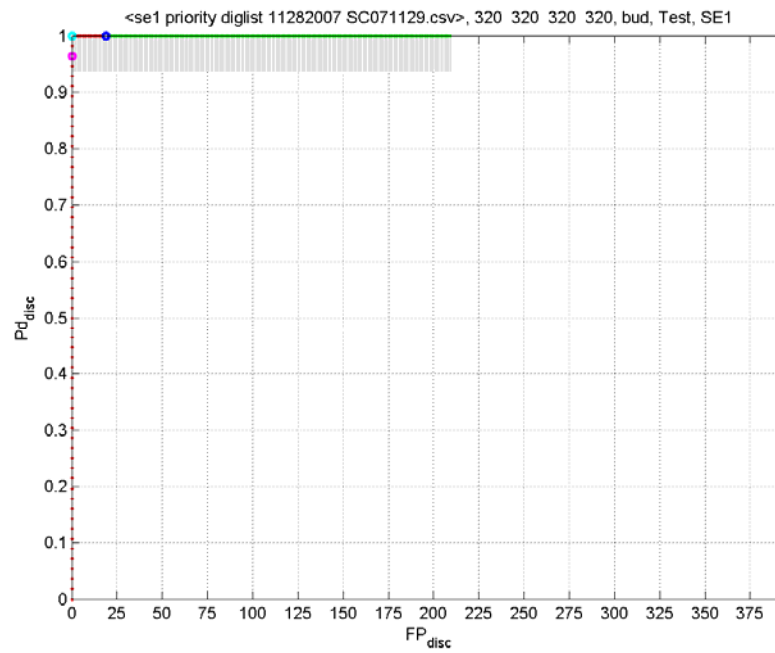
Figure 18: ROC curve for SE1 area for the first priority dig list.
