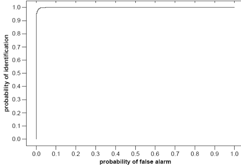
Figure 20: Estimated ROC curve for cued targets priority dig list.
