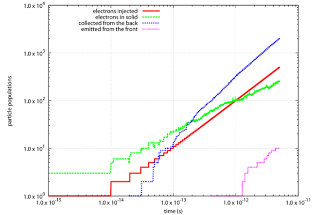
Figure 3. EMC results that showing the collection of air discharge electrons in the rutile. The energetic electrons create approximately two electron-hole pairs in the rutile by impact ionization. A very small fraction of these electrons is emitted.
