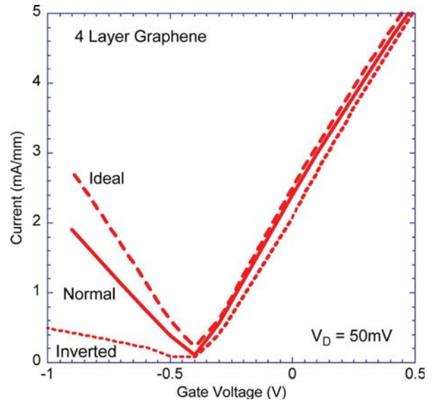
Fig. 11. DD simulation of the total current in a four-layer zero-gap graphene FET as a function of gate voltage.
