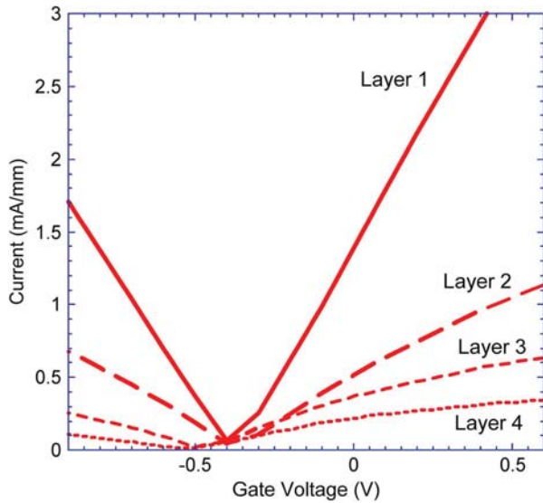
Fig. 10. DD simulation of the current contributions from the individual layers in a four-layer graphene FET as a function of gate voltage. In this simulation, all the layers are assumed to have zero bandgap.
