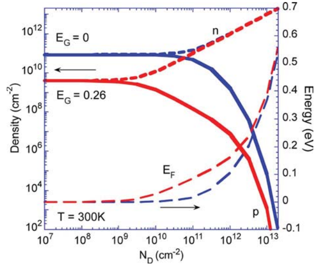
Fig. 1. Electron and hole densities and the Fermi energy versus the doping density in single-layer graphene both with the ideal zero-gap band structure and with a bandgap of 0.26 eV.
