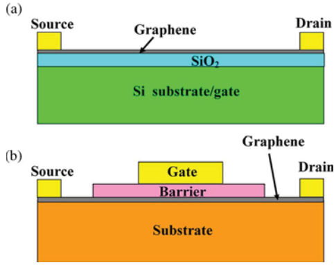
Fig. 5. Depictions of graphene field effect transistors simulated in this paper. (a) Model for the back-gated device studied in [5] and [6]. (b) Model for a front-gated device such as those formed on SiC substrates.
