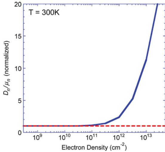
Fig. 4. Enhancement factor for diffusion in graphene due to its bandstructure.
