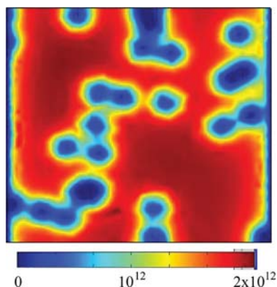
Fig. 12. Electron density in a channel with randomly positioned fixed charges in a 2-D/3-D DD graphene simulation. The region shown is 50 \text{ nm} \times 50 \text{ nm} in size.
