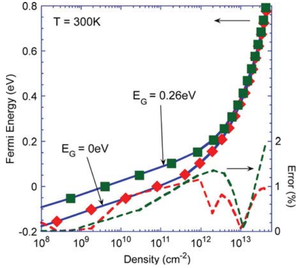
Fig. 3. Variation of the electron density as a function of either the exact chemical potential (lines) or the approximation of (8) for ideal graphene (diamonds) and graphene with a bandgap of 0.26 eV (squares). The relative errors in each case are also shown.
