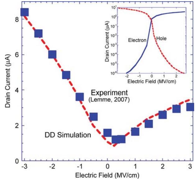
Fig. 6. Experimental data of [5], [6] and fit using a 1-D/2-D DD simulation, as discussed in the text. The inset shows the simulated electron and hole currents in the device.
