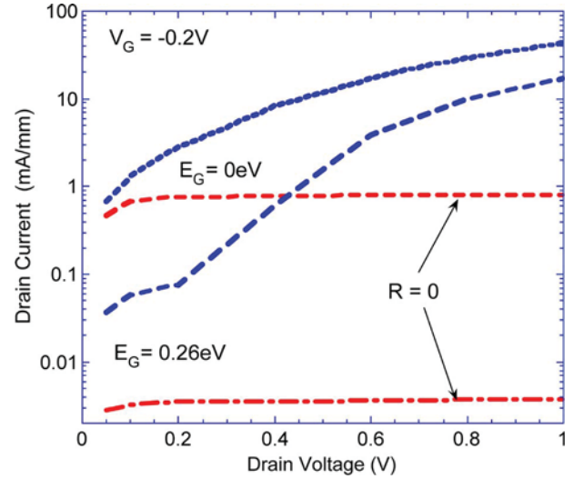
Fig. 9. Drain characteristics with and without carrier generation-recombination and showing the effect of the bandgap in reducing multiplication.
