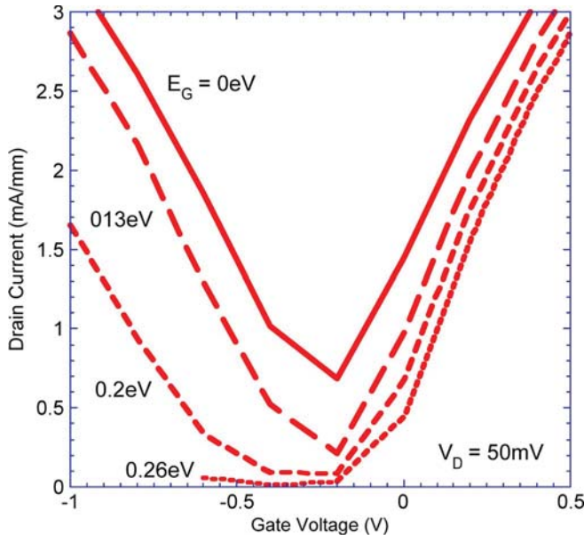
Fig. 7. DD simulation of the effect of a bandgap on the I - V characteristics of a single-layer graphene FET, with L = 0.5 \mu\text{m} and V_D = 50 \text{ mV} .
