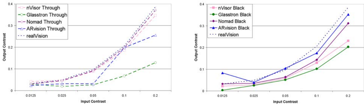
Figure 2: Contrast measurements for the display conditions used in the acuity and contrast experiment as a function of the theoretical (input) contrast. (Left) See-through conditions and realVision condition. (Right) Looking at graphics on a black background and realVision condition.
