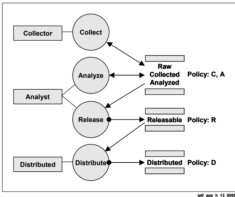
Figure H-13. Structured Analysis Model
