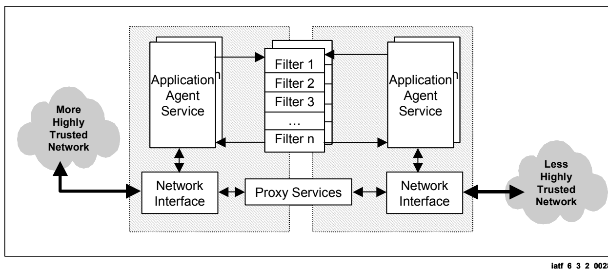
Figure 6.3-2. Dual Network Approach
