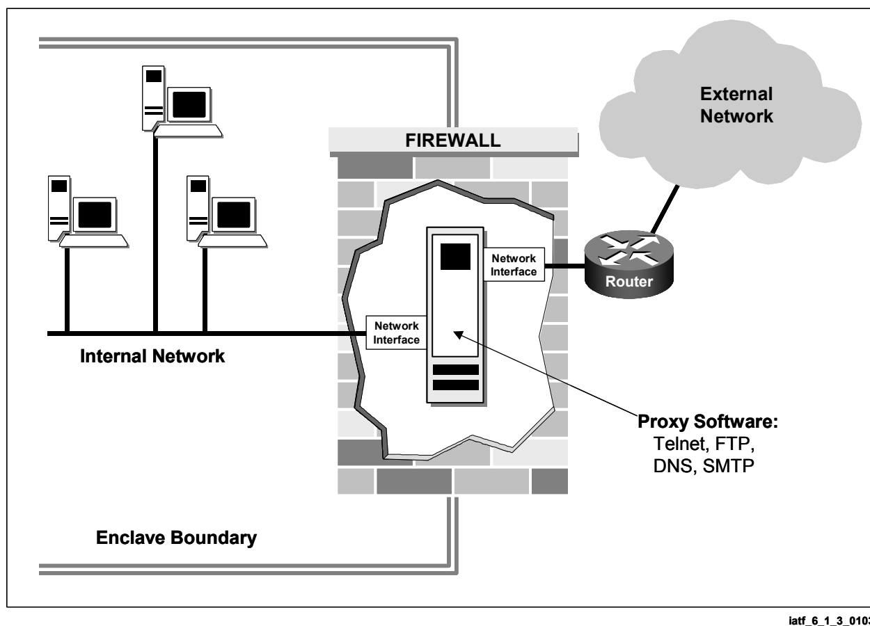
Figure 6.1-3. Dual-Homed Firewall Architecture
