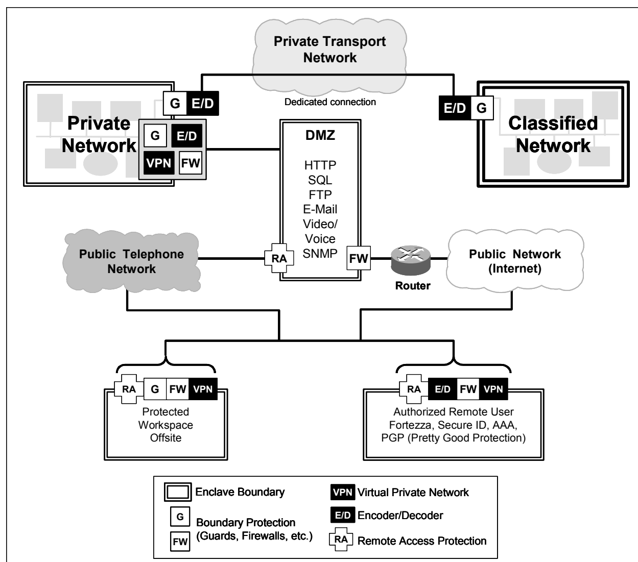
Figure 6.3-1. Guard Environment
