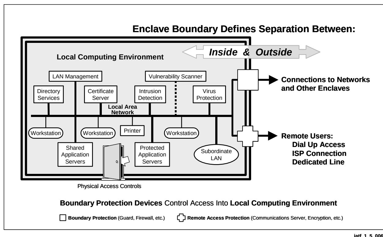
Figure 1-5. Enclave Boundaries Framework Area
