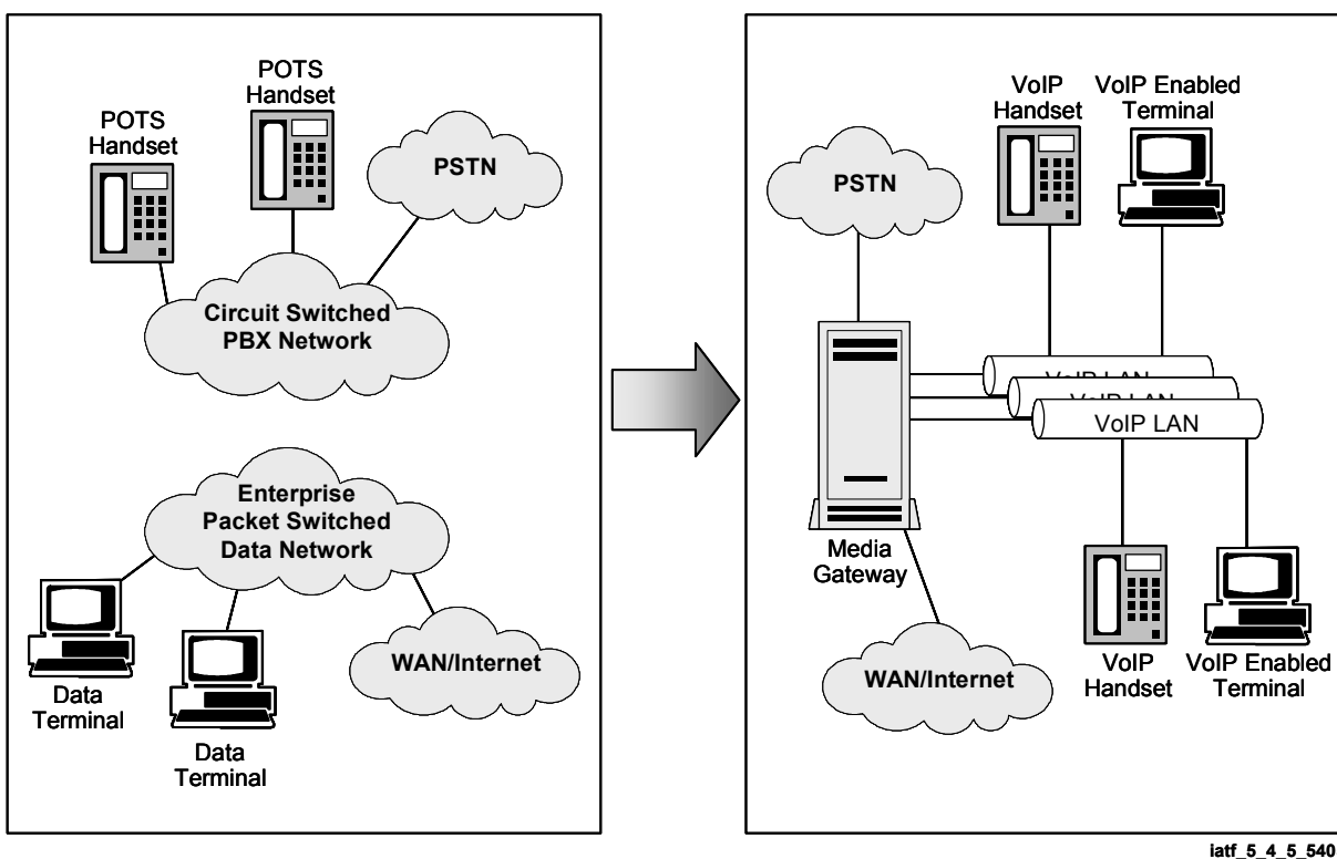
Figure 5.4-5. Integrating a VoIP Capability onto an Existing Network
