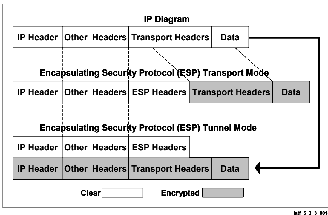
Figure 5.3-3. IP Layering Encryption Methods
