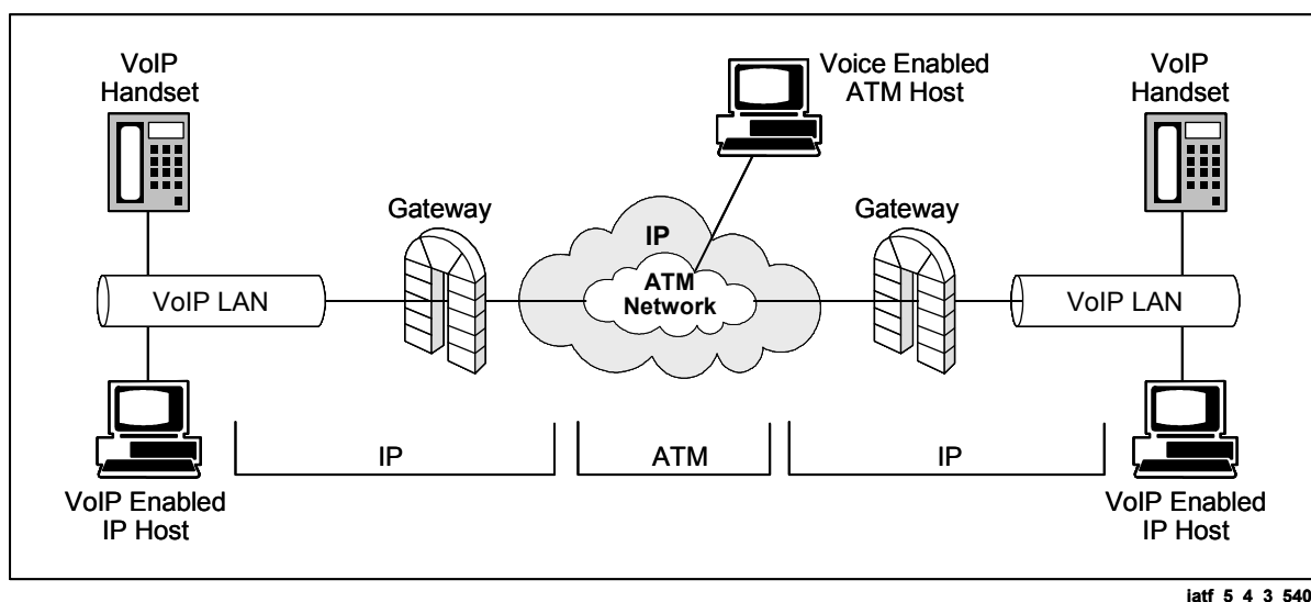
Figure 5.4-3. Voice over ATM
