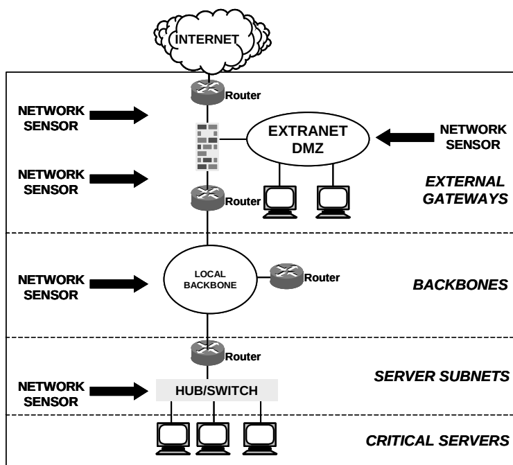
Figure 6.4-2. Network IDS Deployment Options
