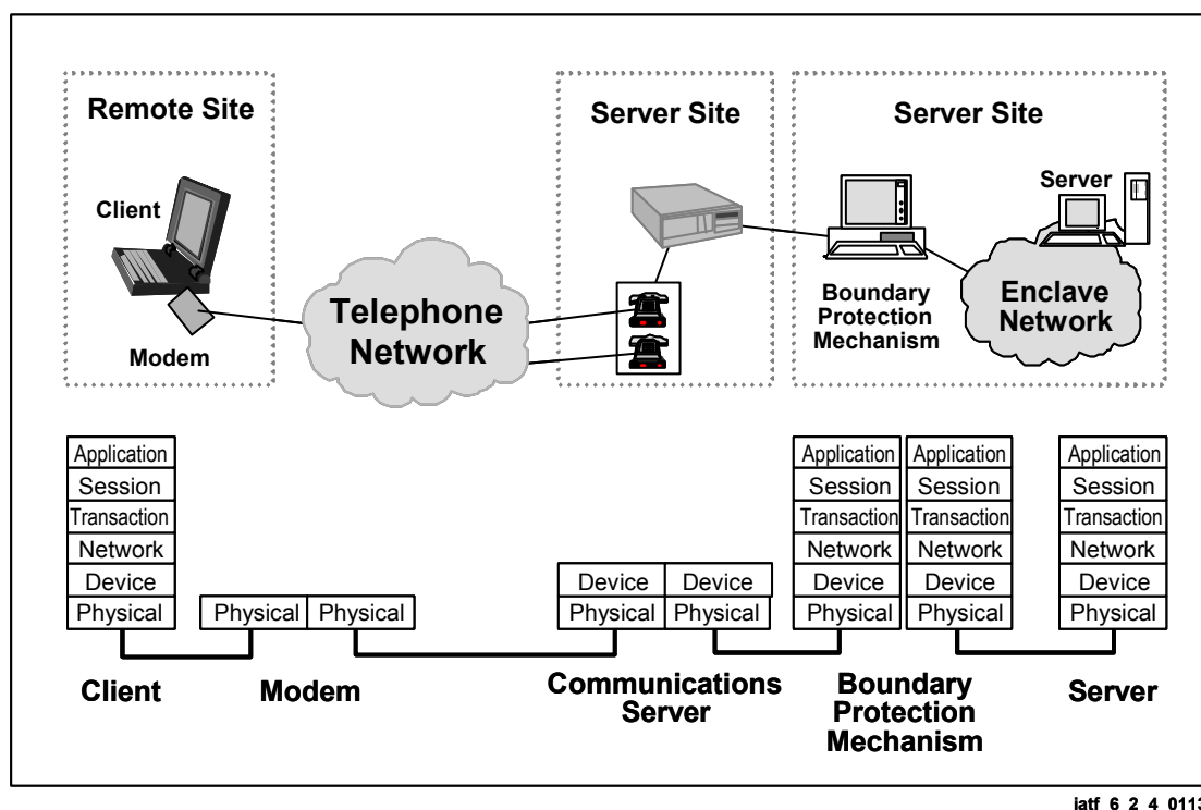
Figure 6.2-4. Protocol Layers In Remote Access Scenario
