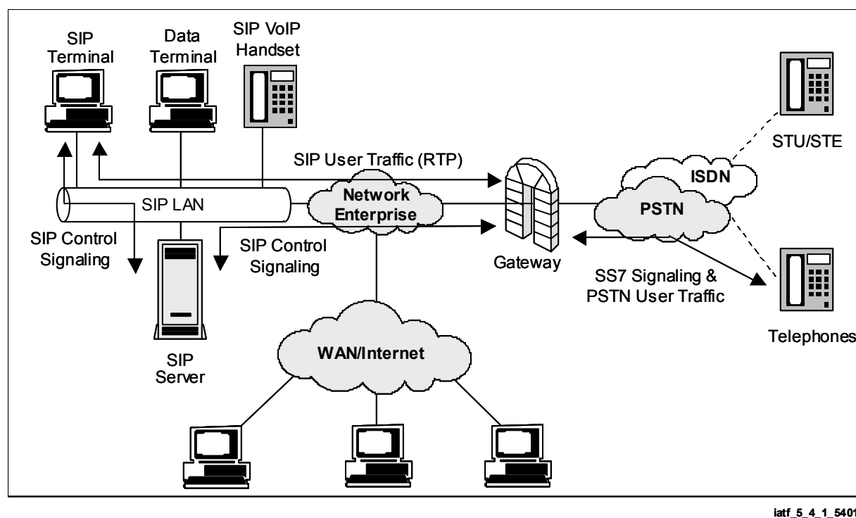
Figure 5.4-1. SIP Network
