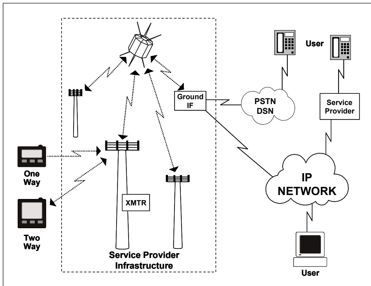
Figure 5.2-5. Pager Environment
