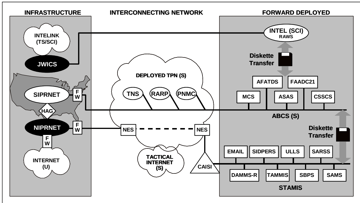
Figure 9-4. Near-Term Architecture [11]
