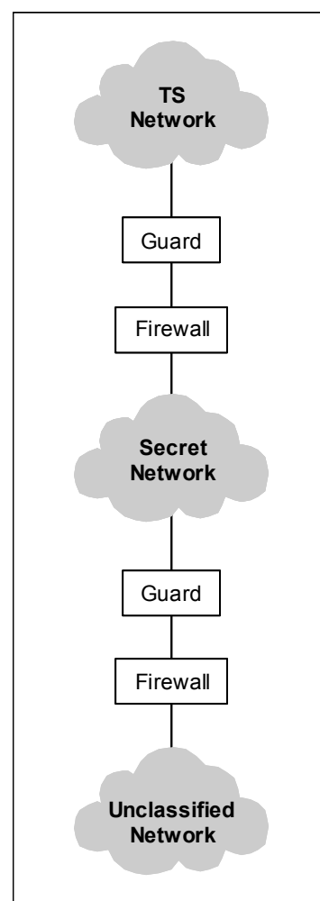
Figure 6.3-3. Cascading Protection
