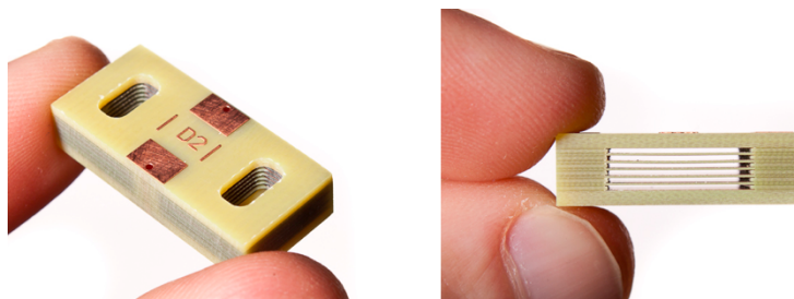
Figure 1: Fabricated MINERVA (Multichannel INtegrated ER Valve Assemblies).
