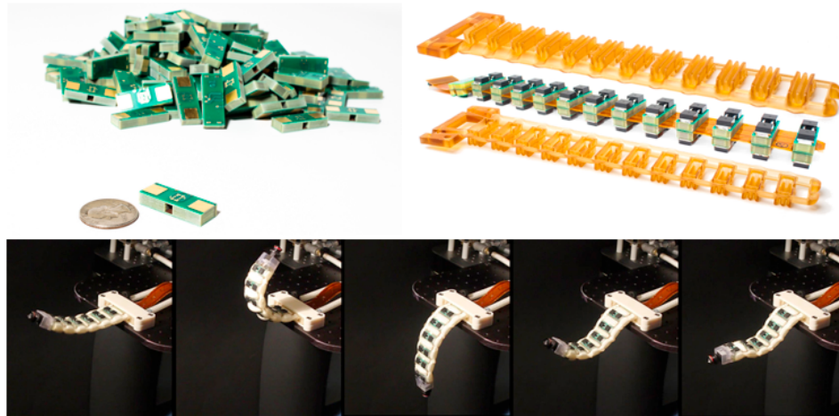
Figure 6: Batch produced MINERVA for ER tentacle. Exploded view of spine construction. Urethane shells (top and bottom) create the flexible actuators and fluid paths, while valving is controlled by the MINERVA along the spine (middle). Screenshots from a demonstration video of 6-segment tentacle motion. Large amplitude upward and downward bending is shown, followed by holding a specific curved shape while moving the camera segment to scan the camera up and down.
