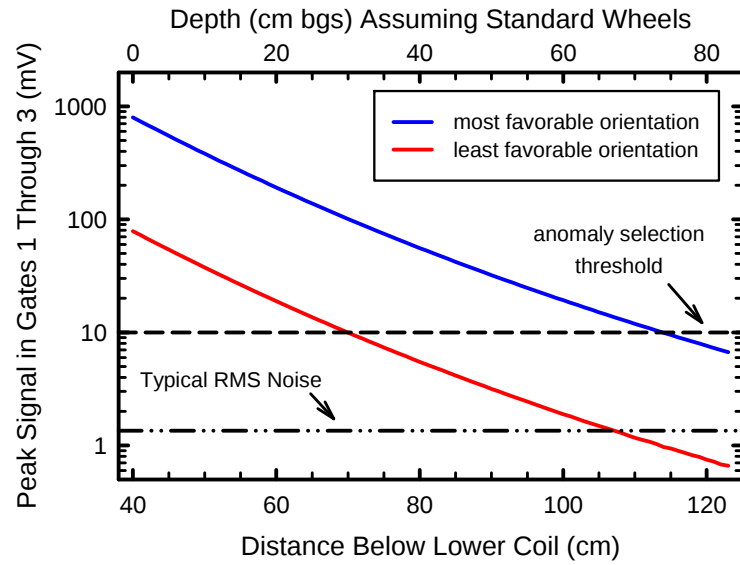
Figure 4-1. Sum of EM61-MK2 response in Gates 1 through 3 versus depth for a small ISO
