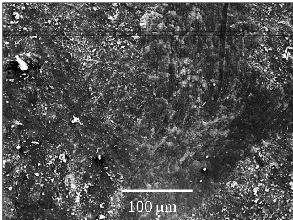
Figure 14. JA2 surface at 100× magnification showing Bi droplet particles and erosion areas from gases moving from reaction site.
