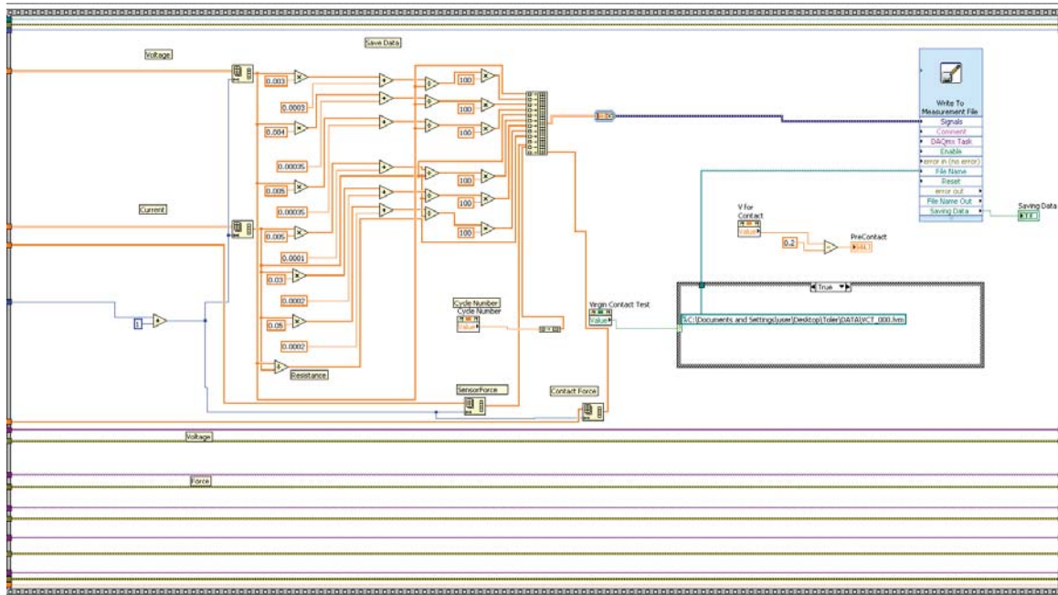
Figure 11 Frame 7 of the Graphical Programming for the Automated Data Acquisition System
