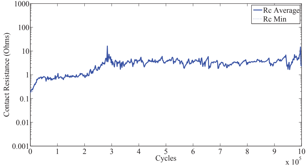
Figure A.49: Contact resistance of Au-Au 6μm radius contact for a 10^6 cycles. 'Rc Average' is the average for the last 5 resistance measurements at \sim 200\mu N of contact force. 'Rc Min' is the minimum contact resistance measured.
