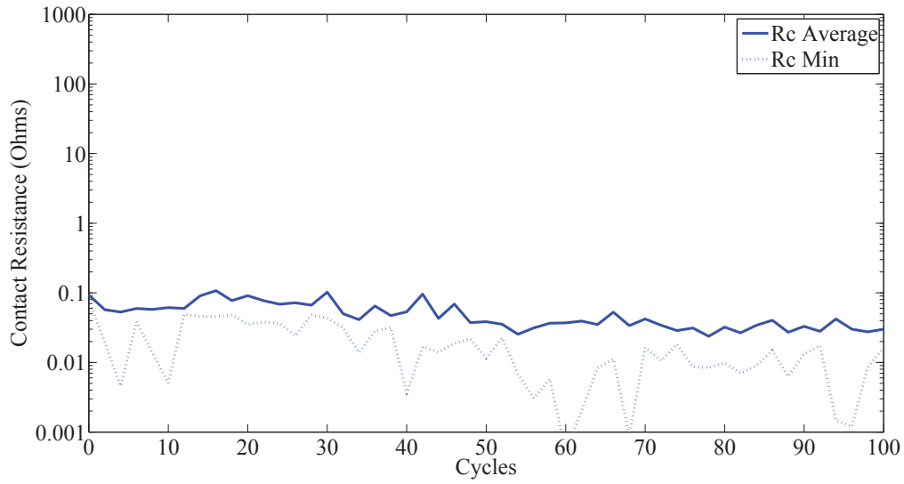
Figure A.25: Contact resistance of Au-Au 6\mu\text{m} radius contact for 100 cycles. Rc Average is the average for the last 4 data point at \sim 200\mu\text{N} of contact force. Rc Min is the minimum contact resistance measured during the measurement cycle
