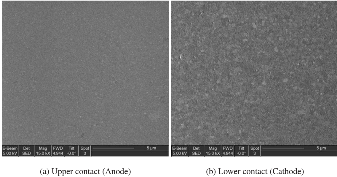
Figure 4.8: Scanning electron microscope image of contact pad after 5 \times 10^5 actuations. No material transfer is shown.
