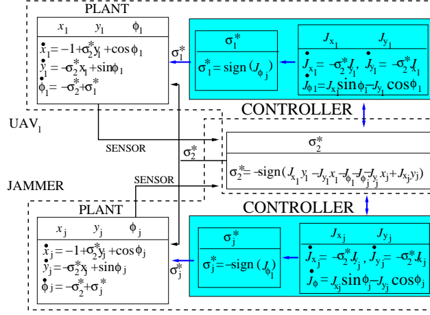
FIGURE 3. The Control Loop for the System
