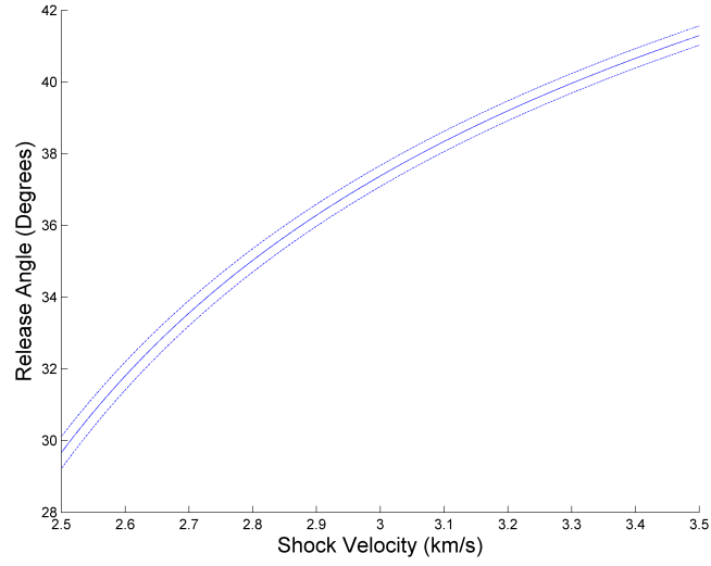
Figure 5. Release angle as a function of shock velocity with 1\text{-}\sigma error over the relevant experimental domain for the wet soil.
