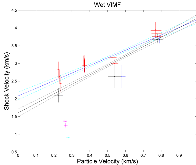
Figure 8. Principal Hugoniot of the wet VIMF. Points shown in red are collected from the pin impedance match, points shown in blue are collected from the VISAR impedance match, and points shown in black are collected from the VISAR wave profile. Error bars are 1-\sigma calculated from the Taylor series method. The points shown in pink and light blue fall on the dry VIMF hugoniot, indicating that the sample lost water before the shot.
