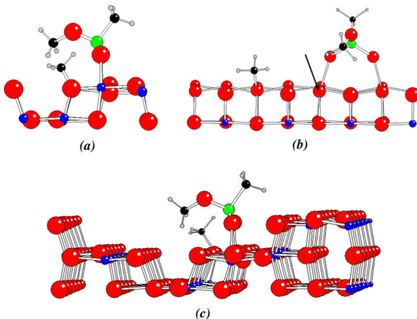
Fig. 4. Similar to Fig. 3 but showing structures considered for the first step in DMMP dissociation. The upper panel shows the unfaceted surface viewed along the (a) [1\ 0\ 0] and (b) [0\ 0\ 1] direction. (c) Shows the faceted surface viewed along the [1\ 0\ 0] direction. Possible H-bonding interactions have been omitted for clarity. The arrow in (b) marks an alternative location for the \text{CH}_3 fragment which is discussed in Section 3.3.
