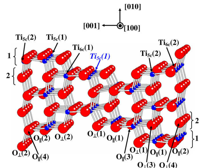
Fig. 2. The faceted surface after relaxation. In correspondence to Table 2, the brackets indicate the layer numbers, and the individual atoms are labeled by type. For clarity, Ti (O) atoms are labeled on the “top” (“bottom”) of the slab. The Layer 1 Ti 5c (2) is obscured by an O atom. The Layer 2 Ti 5c site shown italicized in blue is the one used for DMMP adsorption within the facet (see text). The [0 0 1] and [0 1 0] vectors define the positive directions for Δ x and Δ z , respectively, for the “top” surface atoms (cf. Table 2 and discussion in text). The [0 0 1] and [0 1 0] directions are reversed on the “bottom” surface.
