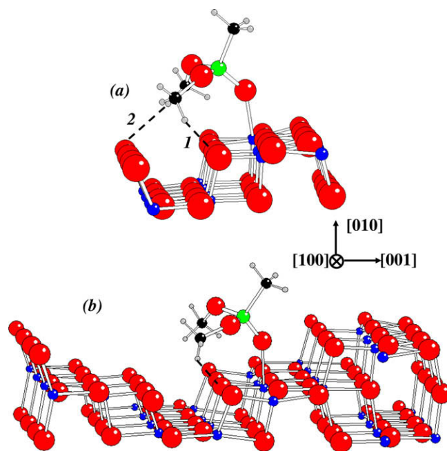
Fig. 3. Sections of the (a) unfaceted and (b) faceted surface after relaxation with adsorbed DMMP in the lowest-energy conformations. For clarity, only sections of the entire slab supercells are shown. The dashed lines show H-bonding interactions identified as such on the basis of the O 2c ···H and O 2c ···C distances and the O 2c ···H—C angle (see text). In (b) the adsorption site is the one designated Layer 2 Ti 5c (1) in Fig. 2. Note that the orientation in (b) is reversed relative to that in Fig. 2. The green, black and gray spheres represent P, C and H respectively. (For interpretation of the references to colour in this figure legend, the reader is referred to the web version of this article.)
