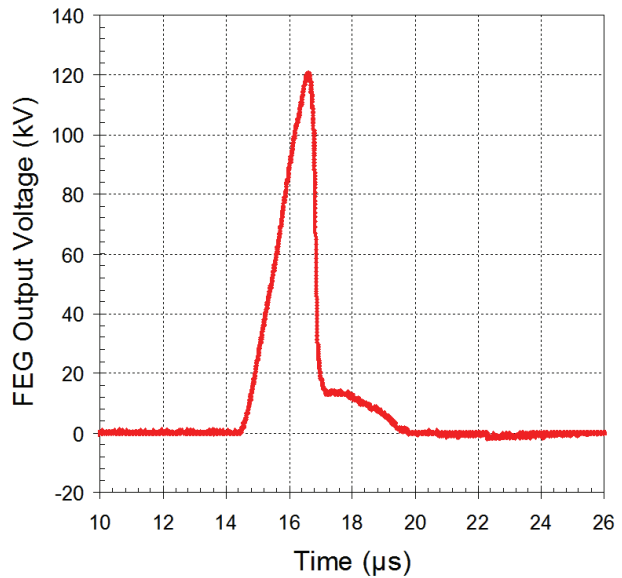
Figure 4. A typical waveform of the output voltage pulse produced by an FEG (38-mm diameter containing PZT 95/5 cylindrical element ( D = 19.0 mm and l = 23.1 mm)).
