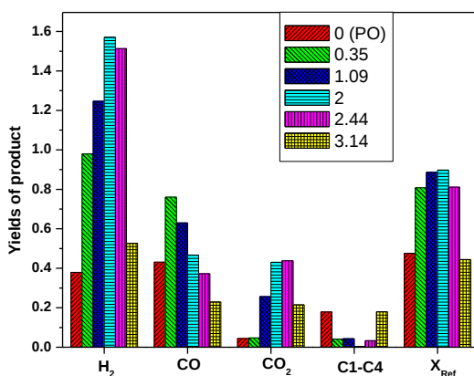
Figure 9. Extent of reforming and product yields during the autothermal reforming of n- dodecane on NCZA catalyst at different H 2 O/C ratios. (Catalyst reduction at 600 °C for 2 h; reaction conditions: Temp: 750 °C; GHSV: 220000 h -1 ; O/C: 0.35)
