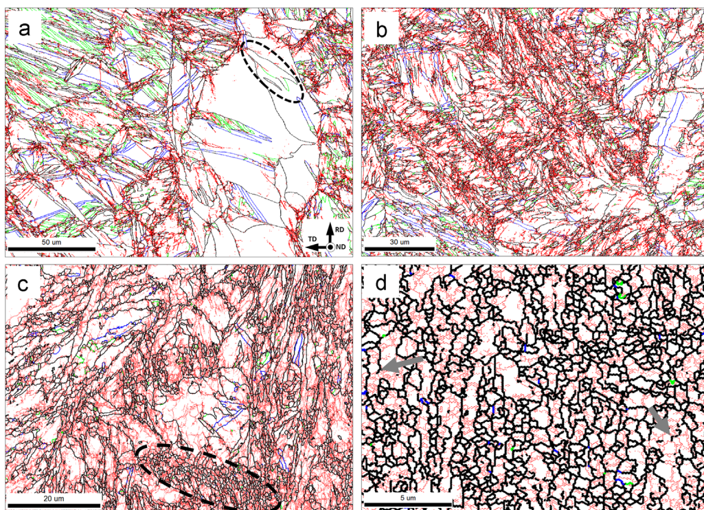
Fig. 4. Selected portions of high-resolution EBSD grain-boundary maps illustrating grain structure which developed after rolling to a reduction of 25% (a), 50% (b), 75% (c), and 96% (d). In the maps, LABs, HABs, 65^\circ\langle 10\bar{1}0 \rangle (compressive twin) and 85^\circ\langle 2\bar{1}10 \rangle (tensile twin) boundaries are depicted as red, black, blue and green lines, respectively. Note difference in scales. The reference frame for all maps is shown in the bottom right corner of (a). (For interpretation of the references to color in this figure legend, the reader is referred to the web version of this article.)
