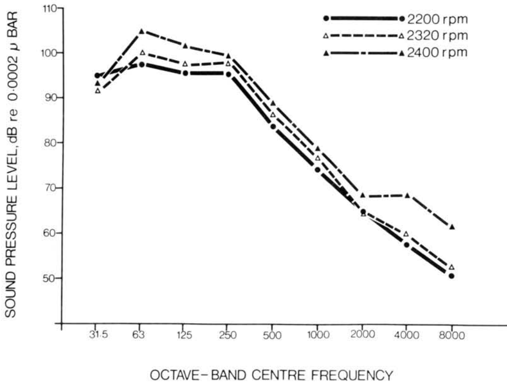
Figure 13. Octave-band sound pressure levels at the MAD Operator location in the Argus aircraft as a function of engine speed.
