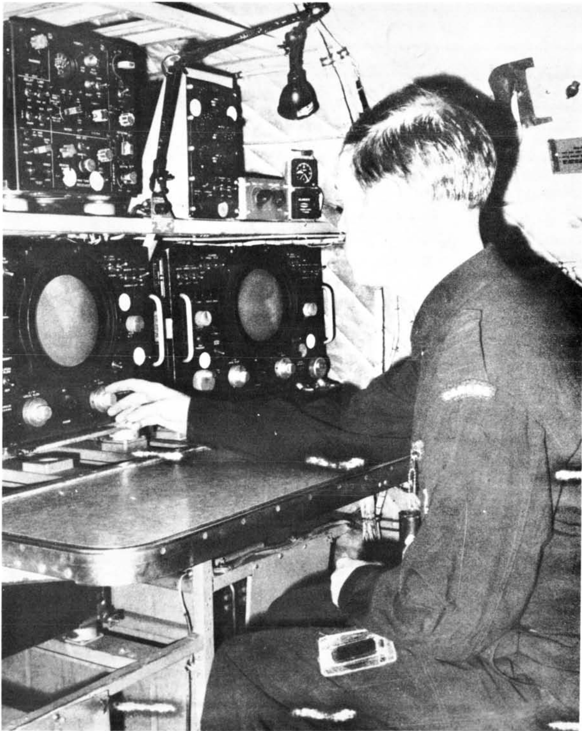
Figure 7. Inadequate table-space and leg-room impose a tiring posture on the radar operator.
