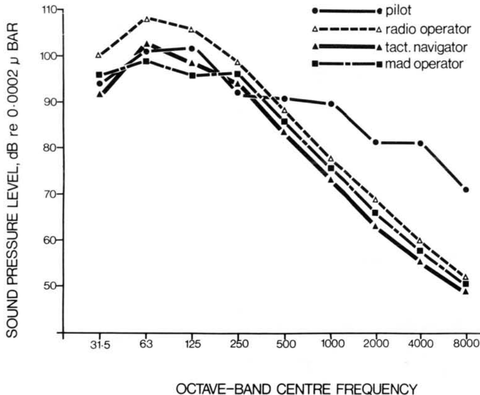
Figure 12. Octave-band sound pressure levels at four crew work locations in the Argus aircraft (engine speed = 2100-2200 rpm).
