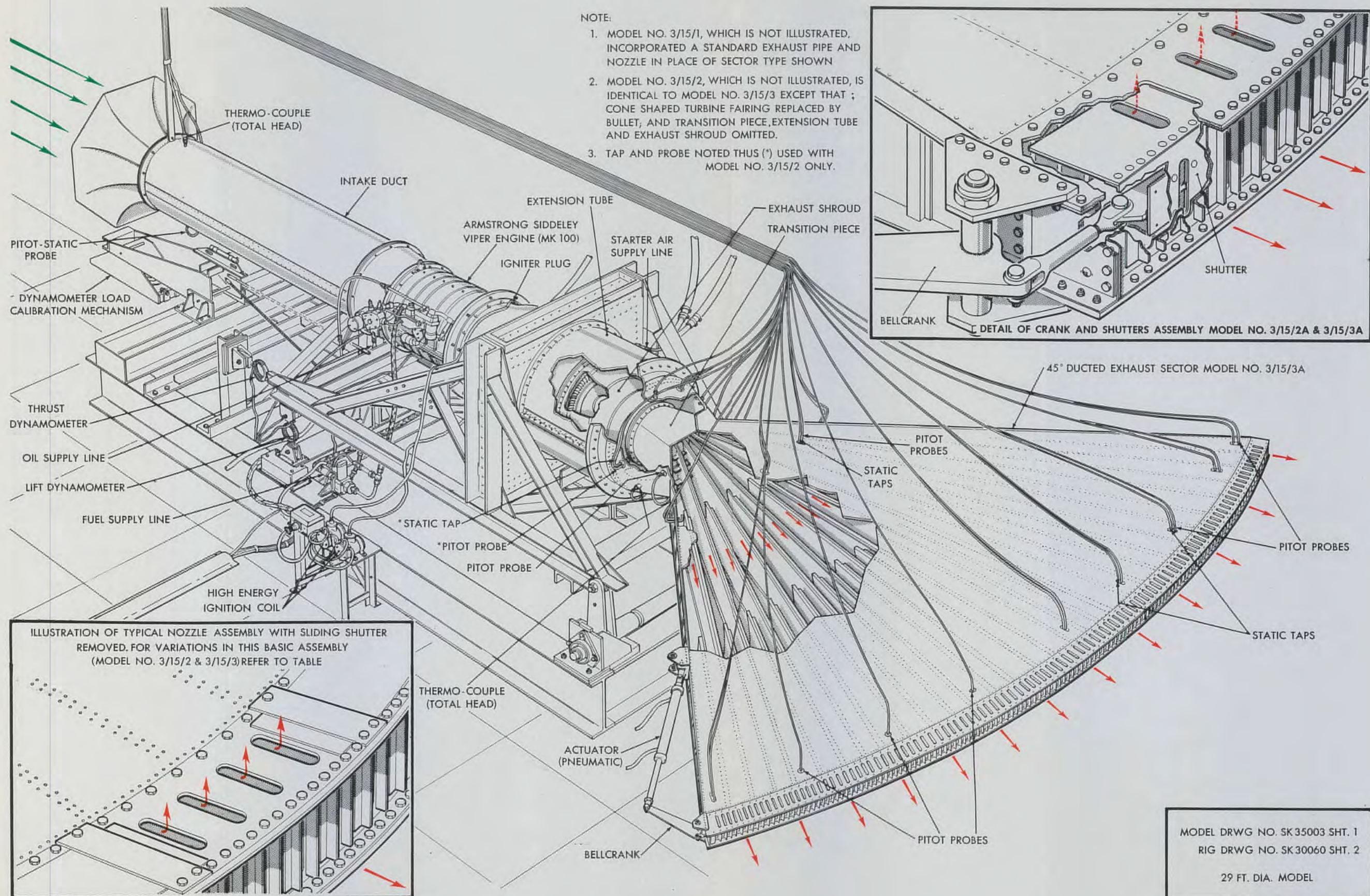
AIR INTAKE AND GAS EXHAUST SYSTEM MODEL NO. 3/15
