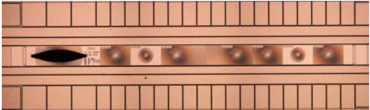
Figure 17: Optical microscope image of active ion trapping zone with nine diffractive optical elements
