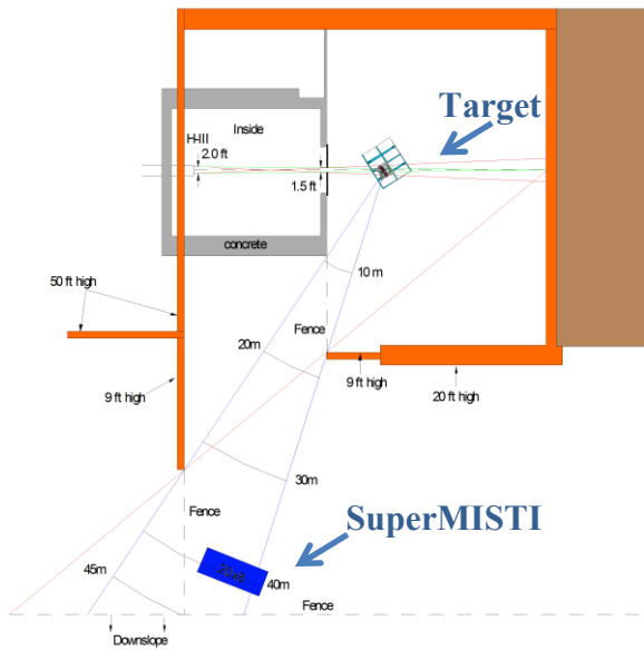
Figure 1. Layout of the Hermes-III test area.
