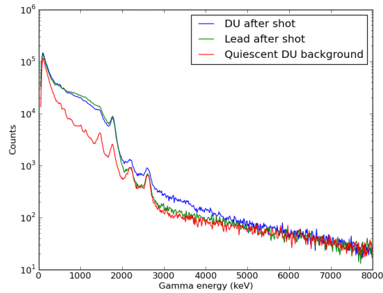
Figure 3. Comparison of gamma spectra measured in NaI detectors for DU and lead targets. Quiescent background denotes spectra for target without interrogating radiation.
