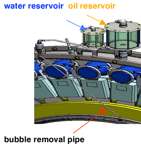
Figure 4. Schematic diagram of a 1-MA LTD cavity section modified in order to operate in a water insulated voltage adder configuration.
