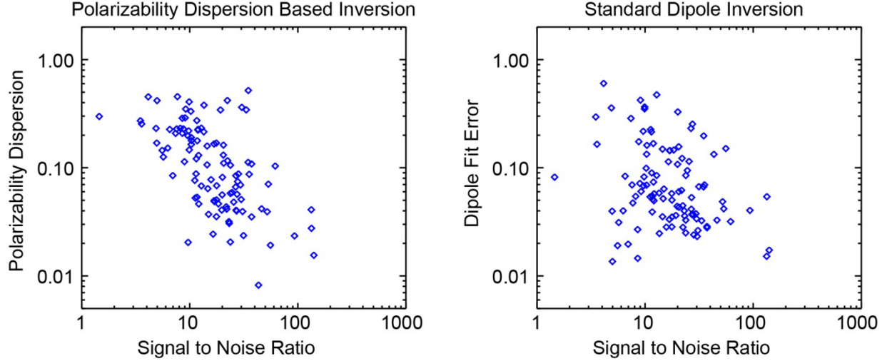
Figure 13. Residual error vs. signal to noise ratio for polarizability dispersion and standard dipole inversion.
