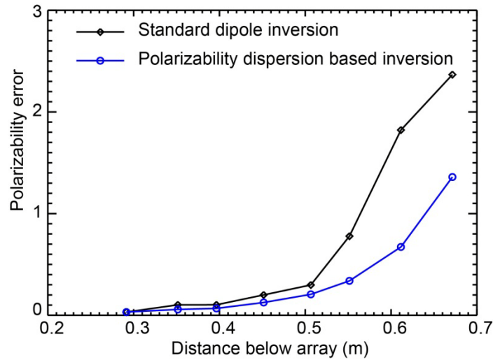
Figure 14. Errors in calculating the polarizability of a 37 mm projectile at various distances below the 2x2 TEM array with standard dipole inversion and polarizability dispersion based processing.
