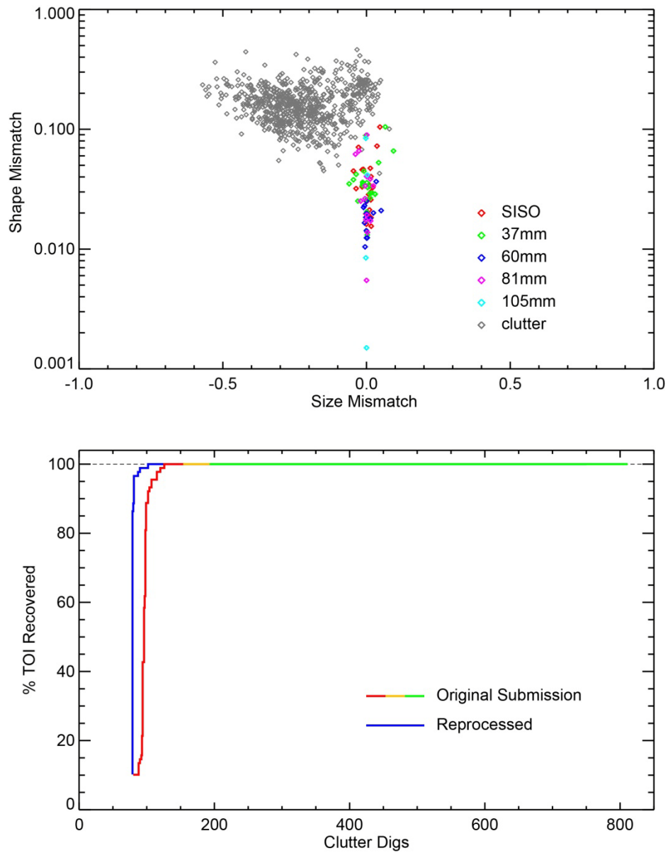
Figure 11. Top: Minimum FOM size and shape mismatch parameters for the targets in the final SAIC Camp Beale dig list. Bottom: ROC curves for the original classification using “traditional” processing (red-orange-green) and re-classification using our new approach (blue).
