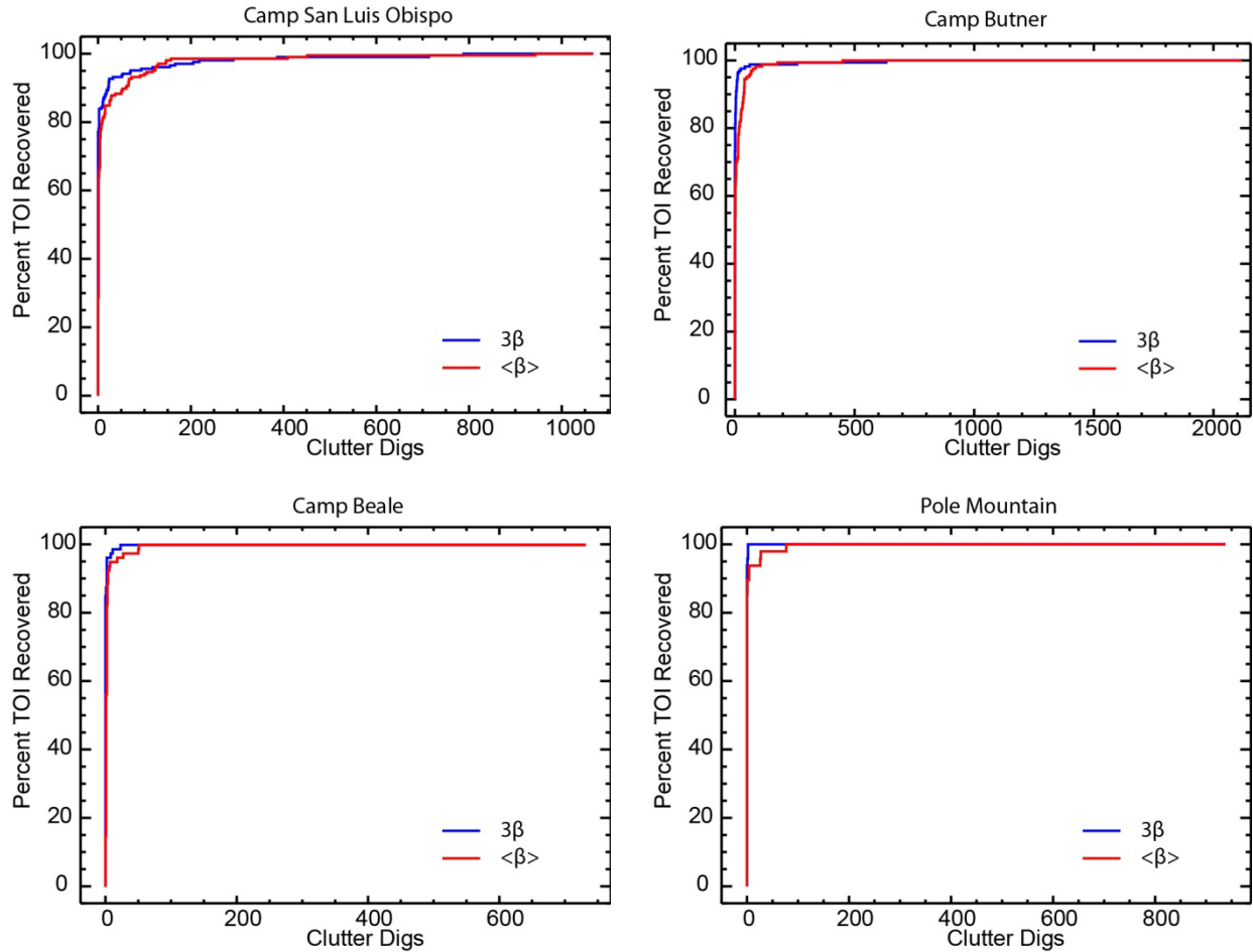
Figure 15. ROC curves for 3\beta and \langle\beta\rangle classification at different ESTCP demonstration sites.
