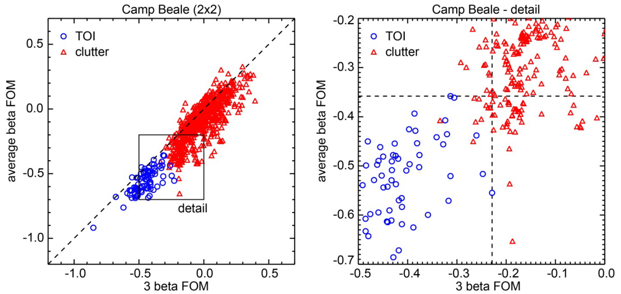
Figure 16. Comparison of target FOM values for classifiers based on all three polarizability eigenvalues and on the average polarizability. Detail on right. Blue circles correspond to munitions items and other targets of interest and red triangles correspond to clutter items.
