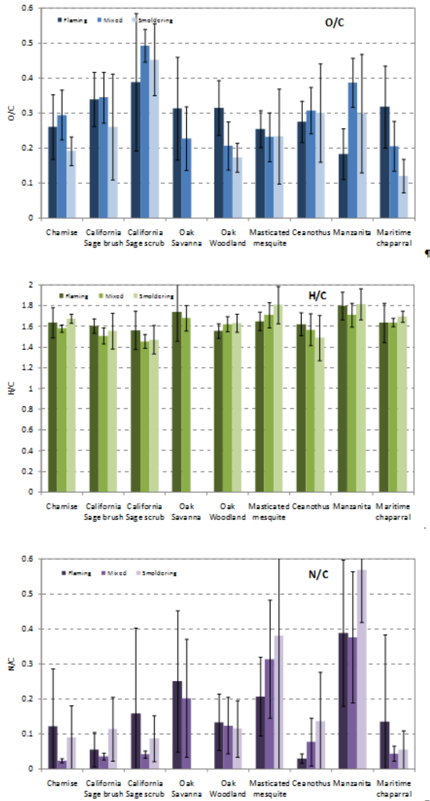
Figure 4-24 Averaged AMS Results showing the Ratio of Various Groups to Carbon (left to right: flaming, transition, smoldering)
