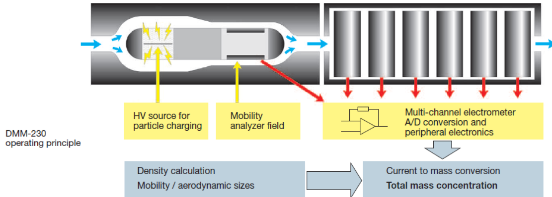
Figure 3-16 Schematic of the Dekati® Mass Monitor
