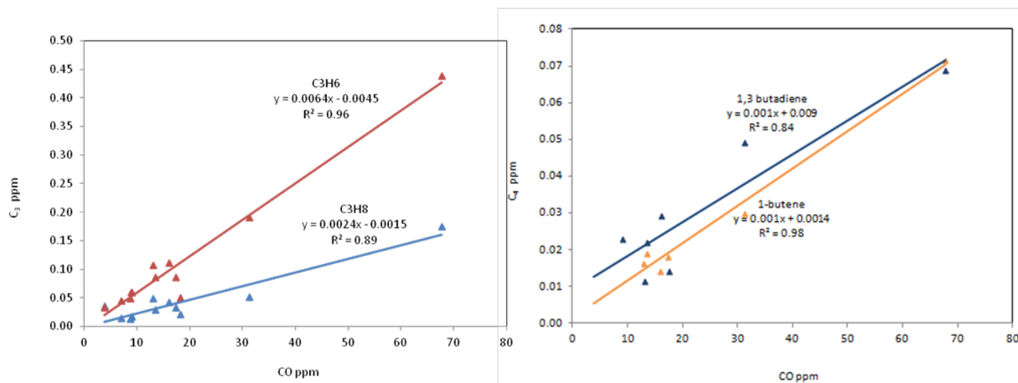
Figure 4-49 Plots of C 3 and C 4 Hydrocarbons vs. CO
