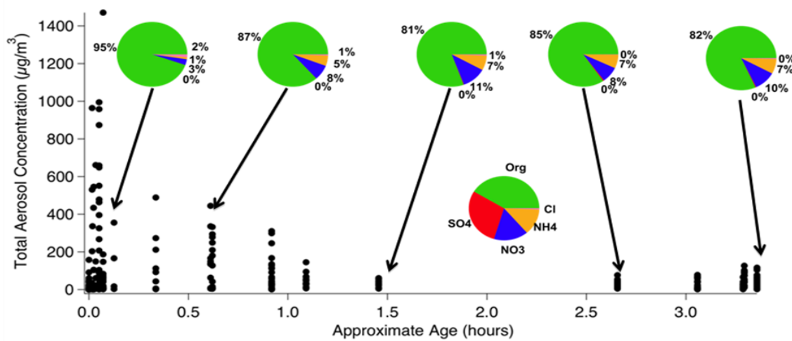
Figure 4-46 In-Plume Aerosol Aging Results from AMS
