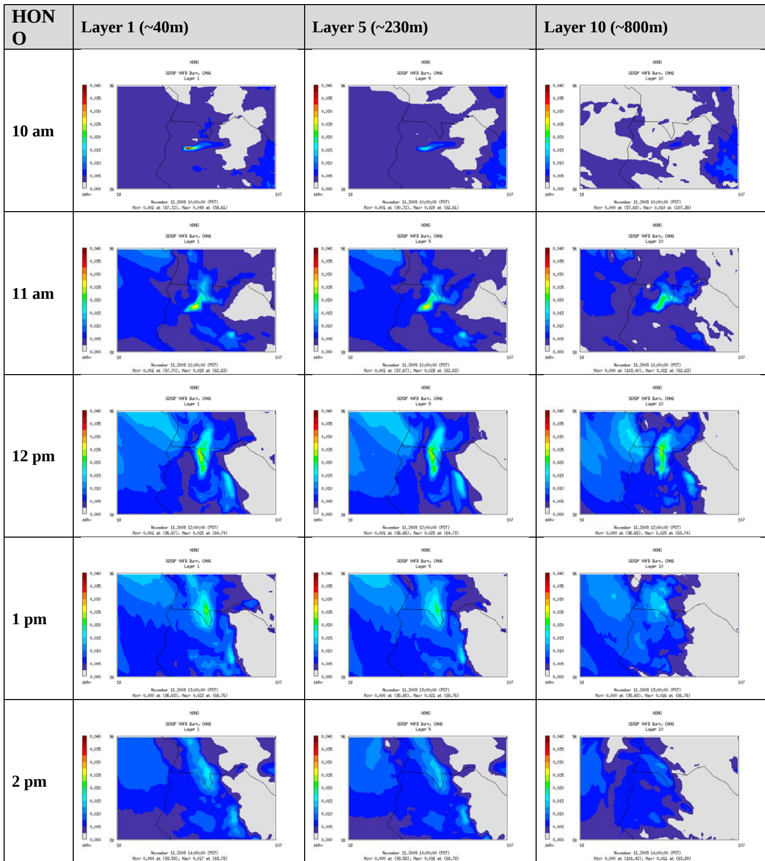
Figure 2e. HONO hourly spatial concentrations at three different vertical layers between 10am to 2pm PST.
