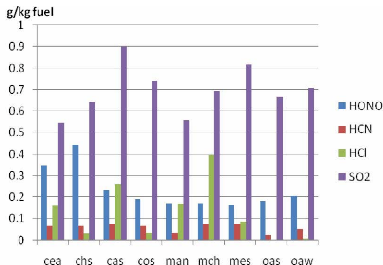
Figure 4-9 Emission Factor for Selected Compounds for some Southwestern Fuel Types
