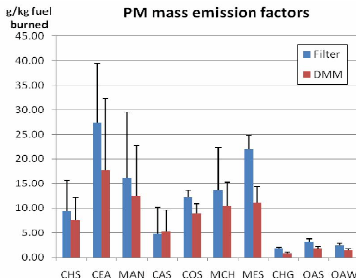
Figure 4-18 PM 2.5 Mass Emission Factor for Different Plant Species
