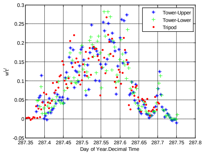
Figure 4-73. Measured Kinematic Sensible Heat Flux at Tower and Tripod Location at Ione
