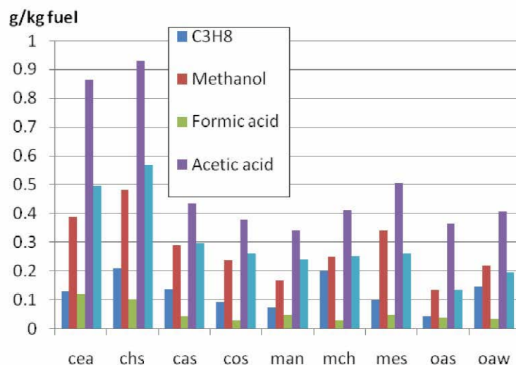
Figure 4-8 Emission Factor of Selected Oxy-Hydrocarbons for some Southwestern Fuel Types
