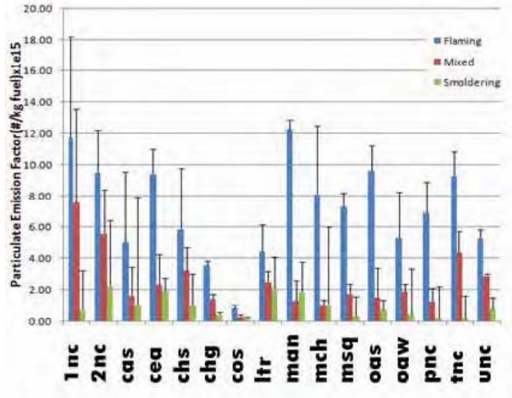
Figure 4-30 Single Burn EFs for Flaming, Mixed and Smoldering Phases for Southeastern and Southwestern Wildland Fuels.
