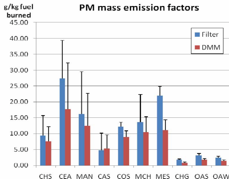
Figure 4-29 PM Emission Factor from a Filter and from DMM
