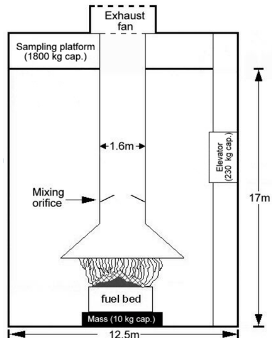
Figure 3-18 Design of Missoula Combustion Lab
