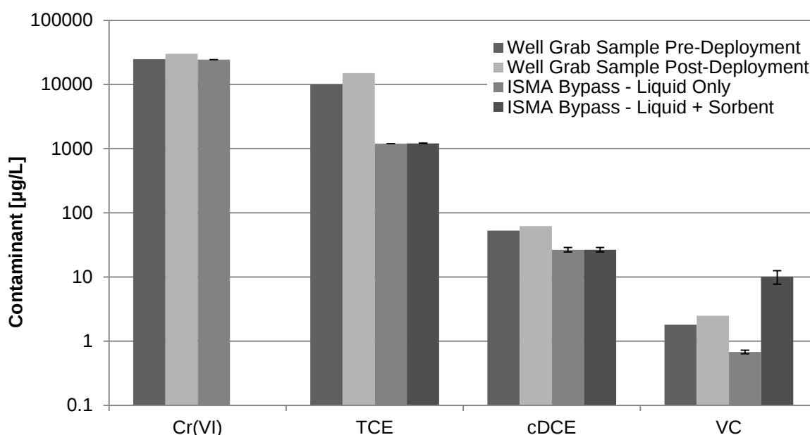
Figure 11. Concentrations of primary contaminants detected in the ISMA deployment well compared to those found in ISMA bypass channels. Error bars represent standard deviation.
