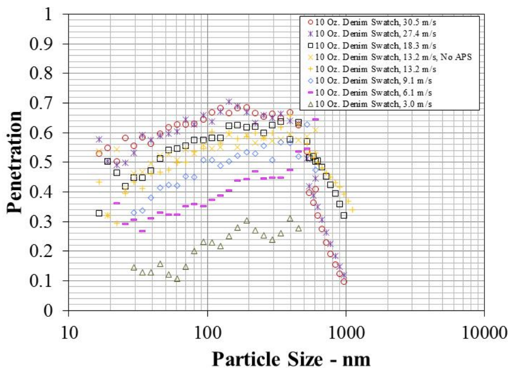
Figure A-33: Wind Tunnel Switch Test, Increasing Face Velocity, DOS Challenge
