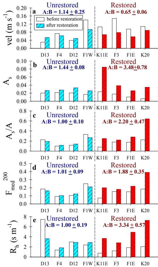
Figure 63. Stream hydrodynamic properties both before (open bars) and after (shaded and hatched bars) CWD additions for each stream: a) surface water velocity (vel, units of m s -1 ), b) size of transient storage zone (A s , units of m 2 ), c) relative size of transient storage zone (A s /A), d) the fraction of the median travel time attributable to transient storage over a standardized length of 200 m (F med 200 ), and e) the hydraulic retention factor (R h , units of s m -1 ). The four control streams are on the left (with blue bars) and the four manipulated (CWD additions) streams are on the right (with red bars) side of each panel. The mean (+ SE) A:B ratio for the control (unrestored) and CWD addition (restored) streams are also indicated in each panel. All differences in A:B ratios were significant between unrestored and restored streams (t-tests on square-root-transformed ratios).
