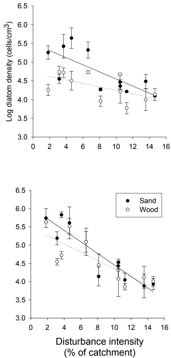
Figure 45. Relationship between catchment disturbance intensity, as indicated by the amount of unpaved road cover or bare ground on slopes >5%) in study catchments, and diatom cell density on stream sand and wood substrates in summer (upper panel) and spring (lower panel) samples (from Miller 2006).
