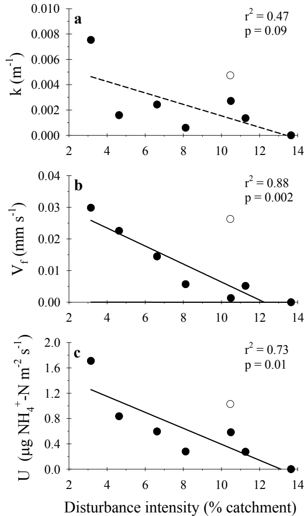
Figure 69. Relationship between catchment disturbance intensity and a) the fractional uptake rate of \text{NH}_4 from water per unit distance ( k ), b) \text{NH}_4 uptake velocity ( V_f ), and c) the mass removal rate of \text{NH}_4 from water per unit area ( U ). The open circle indicates site D12 which was excluded from the statistical analyses. Solid lines are statistically significant ( p < 0.05 ) and dashed lines are marginally significant ( p < 0.10 ) linear regressions and are a) (\text{NH}_4 k) = -0.0005(\text{disturbance intensity}) + 0.0061 , r^2 = 0.47 , p = 0.09 , b) (\text{NH}_4 V_f) = -0.0028(\text{disturbance intensity}) + 0.0348 , r^2 = 0.88 , p = 0.002 , and c) (\text{NH}_4 U) = -0.13(\text{disturbance intensity}) + 1.66 , r^2 = 0.73 , p = 0.01 .
