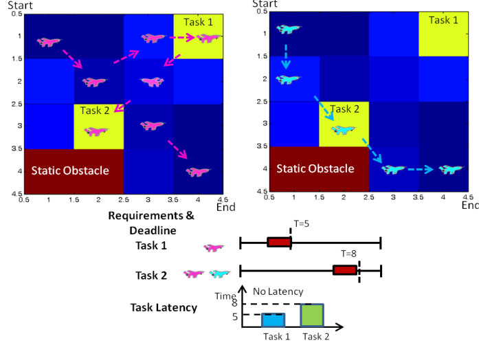
Figure 2: UAV Path Planning Results with static obstacles (Scenario I (a))
