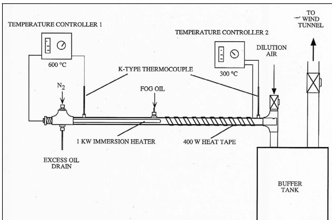
Figure 4. Temperature-Controlled FO Aerosol Generator
