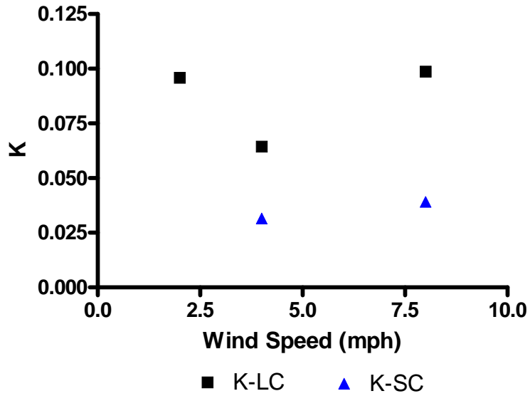
Figure 27. Exponential Decay Coefficient (K) for Each Wind Speed and Canopy Size Using Moth Control Data (LC= large leaf-area canopy, SC = small leaf-area canopy).
