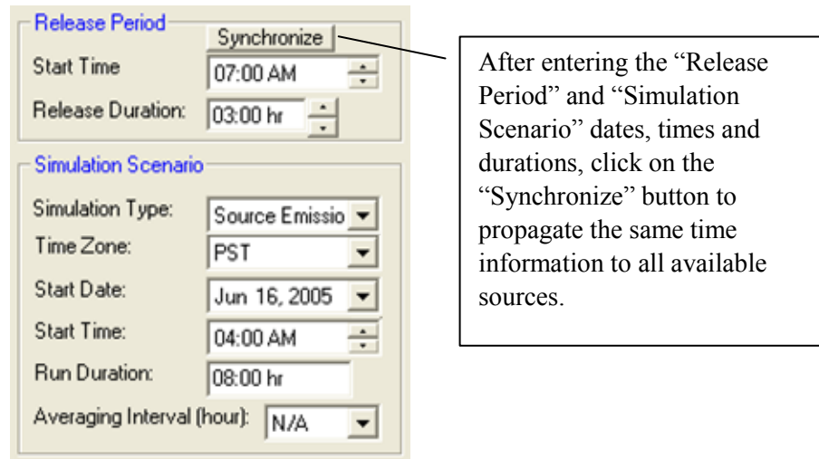
Figure 4.18. Portion of Main DUSTAN Control Panel
